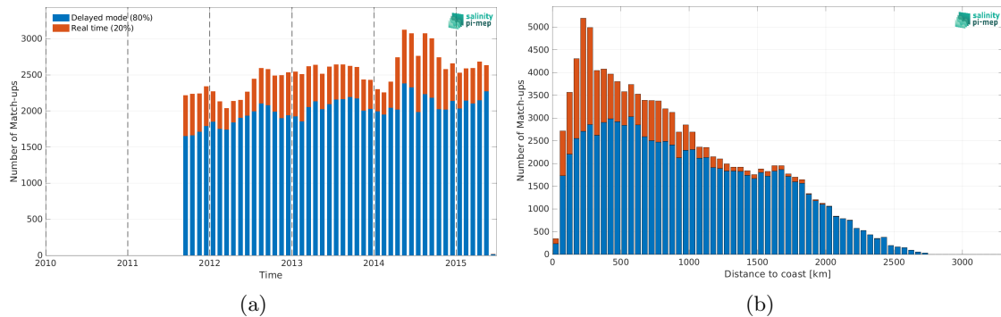
Figure 1: Number of match-ups between Argo and Aquarius SSS L4 OI v5 - Monthly (IPRC) SSS as a function of time (a) and as function of the distance to coast (b) over the North Pacific Ocean Pi-MEP region and for the full satellite product period.
