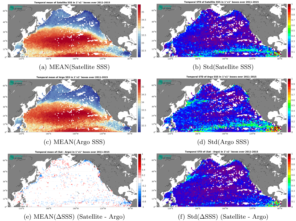
Figure 6: Temporal mean (left) and Std (right) of SSS from Aquarius SSS L4 OI v5 - Monthly (IPRC) (top), Argo (middle), and of \Delta\text{SSS} (Satellite - Argo). Only match-up pairs are used to generate these maps.
