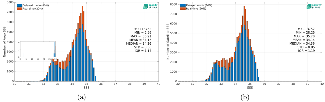
Figure 2: Histograms of SSS from Argo (a) and Aquarius SSS L4 OI v5 - Monthly (IPRC) (b) considering all match-up pairs per bins of 0.1 over the North Pacific Ocean Pi-MEP region and for the full satellite product period.
