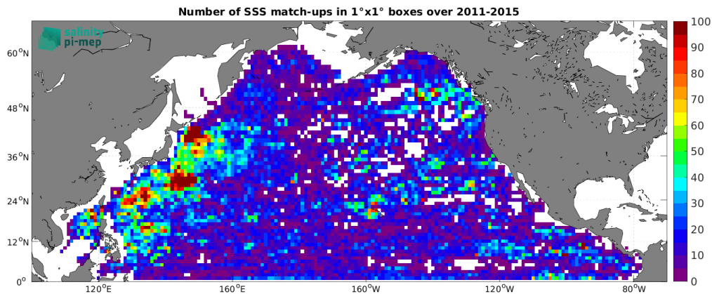
Figure 4: Number of SSS match-ups between Argo SSS and the Aquarius SSS L4 OI v5 - Monthly (IPRC) SSS product for the North Pacific Ocean Pi-MEP region over 1^\circ \times 1^\circ boxes and for the full satellite product period.
