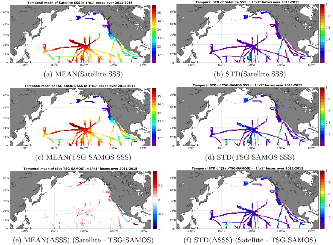
Figure 6: Temporal mean (left) and STD (right) of SSS from Aquarius-L4-IPRC-V4-WEEKLY (top), TSG-SAMOS (middle), and of \Delta SSS (Satellite - TSG-SAMOS). Only match-up pairs are used to generate these maps.
