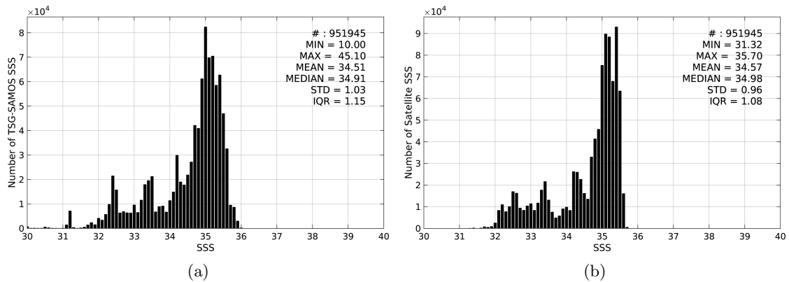
Figure 2: Histograms of SSS from TSG-SAMOS (a) and Aquarius-L4-IPRC-V4-WEEKLY (b) considering all match-up pairs per bins of 0.1 over the North Pacific Ocean Pi-MEP region and for the full satellite product period.
