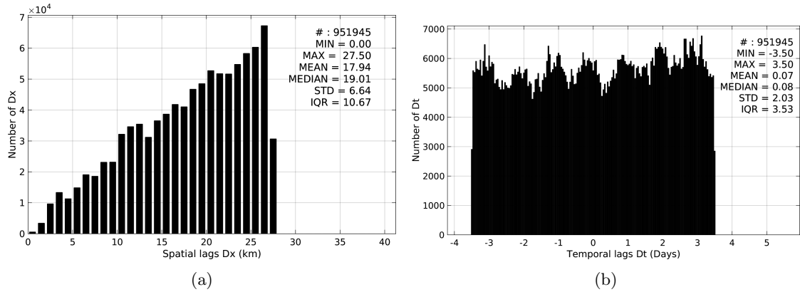
Figure 5: Histograms of the spatial (a) and temporal (b) lags between the time of the TSG-SAMOS measurements and the date of the corresponding Aquarius-L4-IPRC-V4-WEEKLY SSS product.
