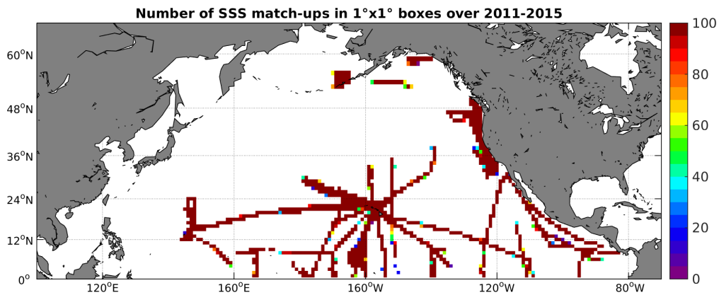
Figure 4: Number of SSS match-ups between TSG-SAMOS SSS and the Aquarius-L4-IPRC-V4-WEEKLY SSS product for the North Pacific Ocean Pi-MEP region over 1^\circ \times 1^\circ boxes and for the full satellite product period.
