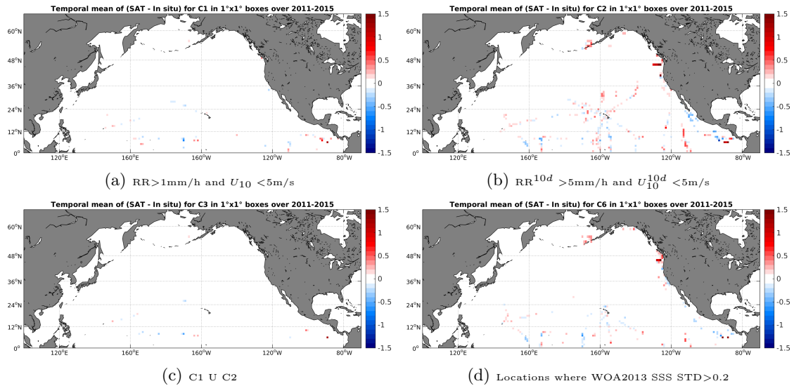
Figure 12: Temporal mean gridded over spatial boxes of size 1^\circ \times 1^\circ of \Delta SSS (Aquarius-L4-IPRC-V4-WEEKLY - TSG-SAMOS) for 4 different subdatasets corresponding to: RR > 1\text{mm/h} and U_{10} < 5\text{m/s} (a), RR^{10d} > 5\text{mm/h} and U_{10}^{10d} < 5\text{m/s} (b), C1 U C2 (c), Locations where WOA2013 SSS STD > 0.2 (d).
