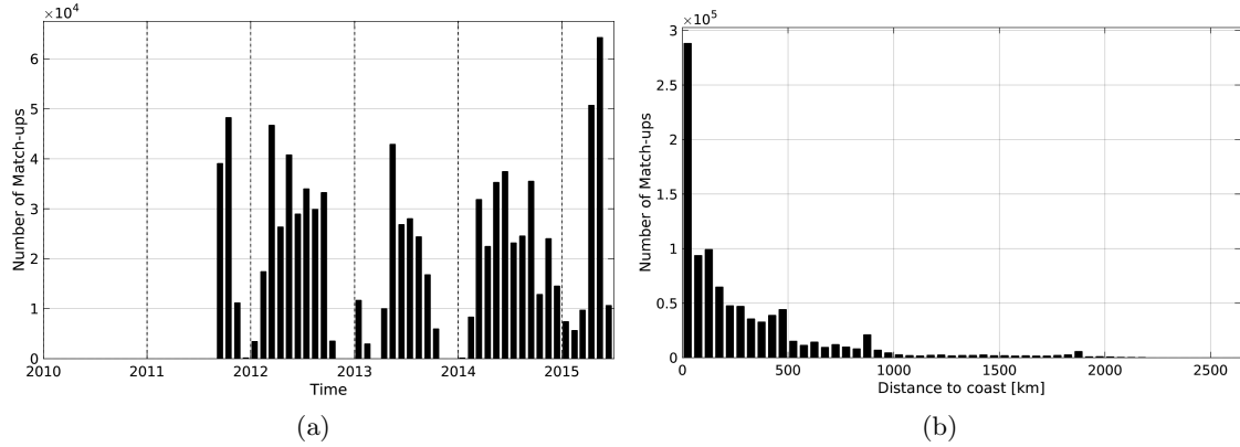
Figure 1: Number of match-ups between TSG-SAMOS and Aquarius-L4-IPRC-V4-WEEKLY SSS as a function of time (a) and as function of the distance to coast (b) over the North Pacific Ocean Pi-MEP region and for the full satellite product period.
