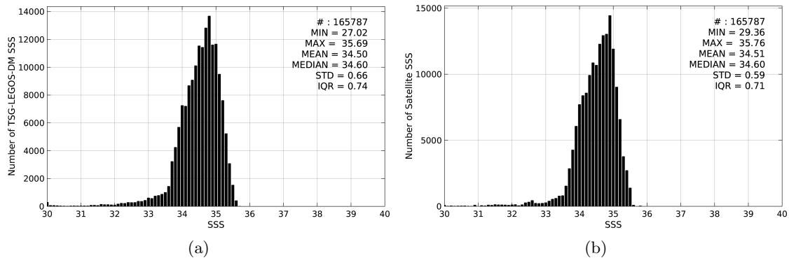
Figure 2: Histograms of SSS from TSG-LEGOS-DM (a) and Aquarius-L4-IPRC-V4-WEEKLY (b) considering all match-up pairs per bins of 0.1 over the North Pacific Ocean Pi-MEP region and for the full satellite product period.
