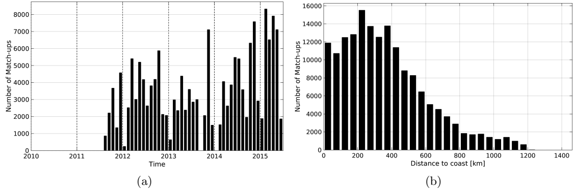
Figure 1: Number of match-ups between TSG-LEGOS-DM and Aquarius-L4-IPRC-V4-WEEKLY SSS as a function of time (a) and as function of the distance to coast (b) over the North Pacific Ocean Pi-MEP region and for the full satellite product period.
