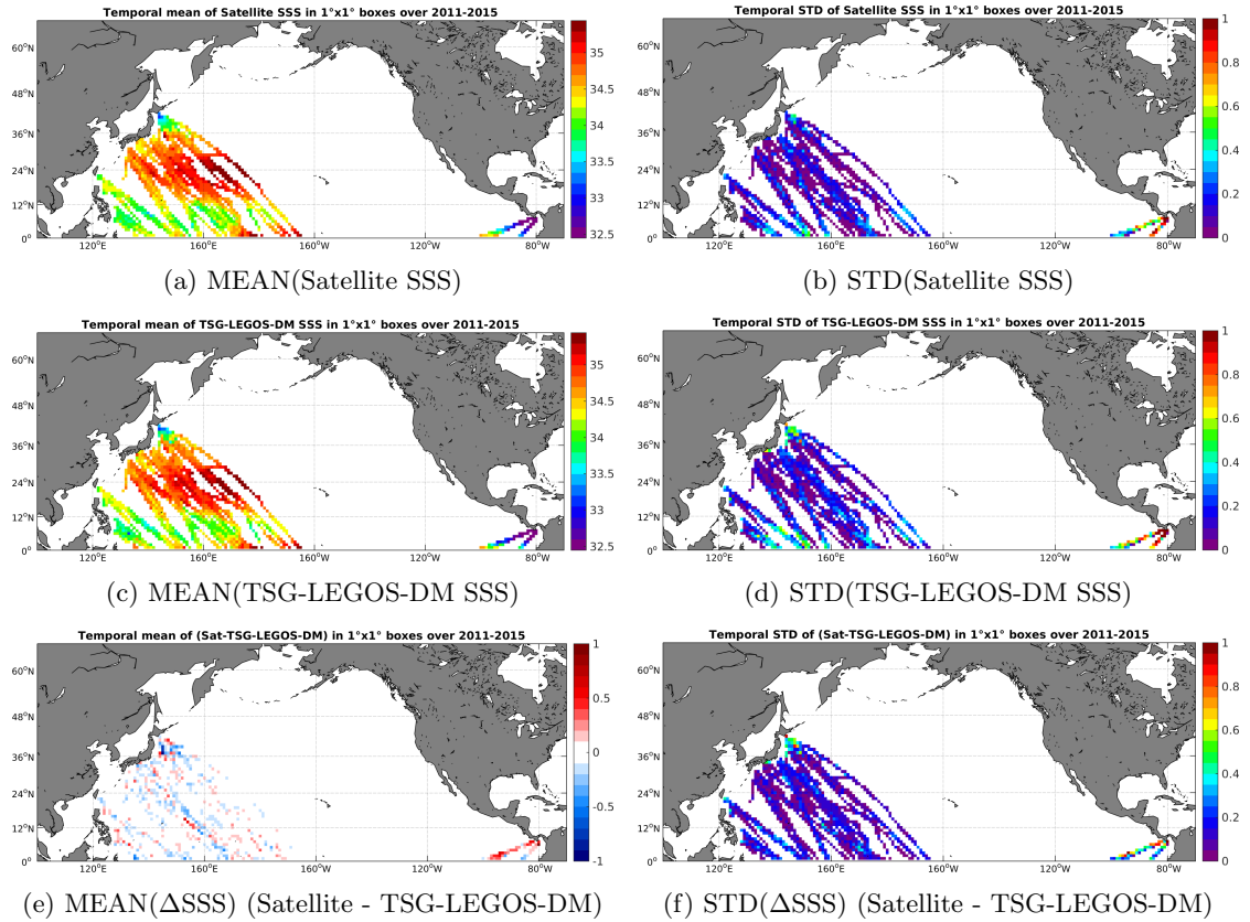
Figure 6: Temporal mean (left) and STD (right) of SSS from Aquarius-L4-IPRC-V4-WEEKLY (top), TSG-LEGOS-DM (middle), and of \Delta SSS (Satellite - TSG-LEGOS-DM). Only match-up pairs are used to generate these maps.
