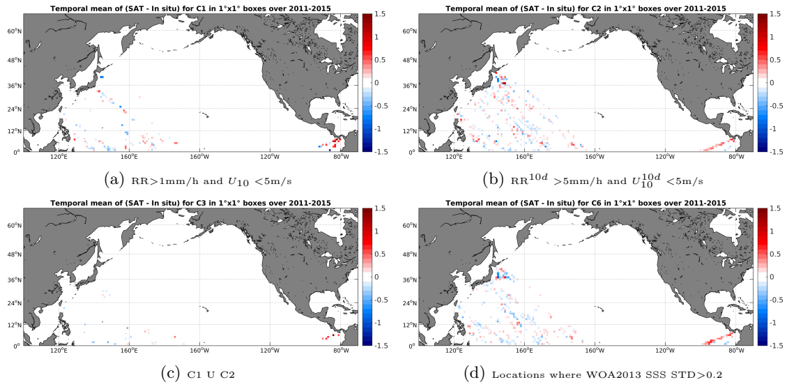
Figure 12: Temporal mean gridded over spatial boxes of size 1^\circ \times 1^\circ of \Delta SSS (Aquarius-L4-IPRC-V4-WEEKLY - TSG-LEGOS-DM) for 4 different subdatasets corresponding to: RR > 1\text{mm/h} and U_{10} < 5\text{m/s} (a), RR^{10d} > 5\text{mm/h} and U_{10}^{10d} < 5\text{m/s} (b), C1 U C2 (c), Locations where WOA2013 SSS STD > 0.2 (d).
