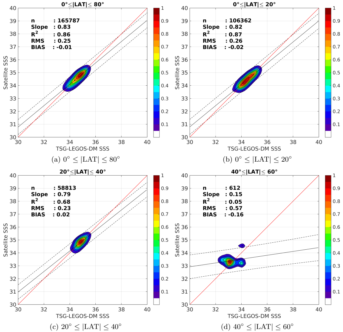
Figure 9: Contour maps of the concentration of Aquarius-L4-IPRC-V4-WEEKLY SSS (y-axis) versus TSG-LEGOS-DM SSS (x-axis) at match-up pairs for different latitude bands. For each plot, the red line shows x=y . The black thin and dashed lines indicate a linear fit through the data cloud and the \pm 95\% confidence levels, respectively. The number match-up pairs n , the slope and R^2 coefficient of the linear fit, the root mean square (RMS) and the mean bias between satellite and in situ data are indicated for each latitude band in each plots.
