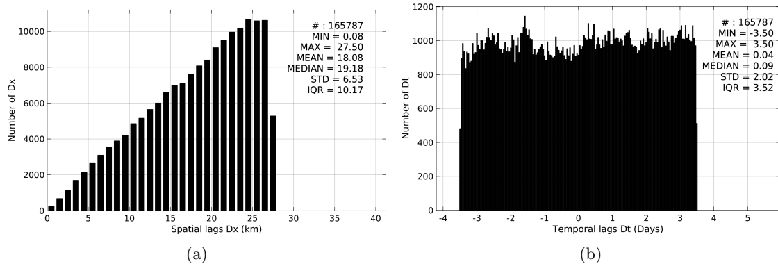
Figure 5: Histograms of the spatial (a) and temporal (b) lags between the time of the TSG-LEGOS-DM measurements and the date of the corresponding Aquarius-L4-IPRC-V4-WEEKLY SSS product.
