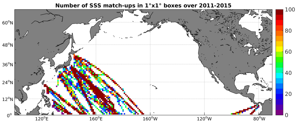
Figure 4: Number of SSS match-ups between TSG-LEGOS-DM SSS and the Aquarius-L4-IPRC-V4-WEEKLY SSS product for the North Pacific Ocean Pi-MEP region over 1^\circ \times 1^\circ boxes and for the full satellite product period.
