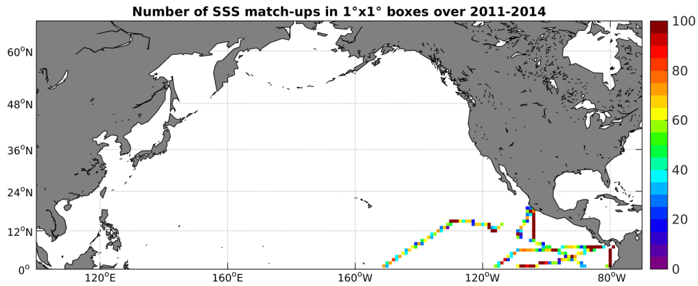
Figure 4: Number of SSS match-ups between TSG-GOSUD-Research-vessel SSS and the Aquarius-L4-IPRC-V4-WEEKLY SSS product for the North Pacific Ocean Pi-MEP region over 1^\circ \times 1^\circ boxes and for the full satellite product period.
