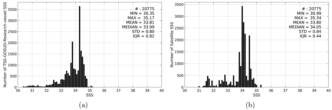
Figure 2: Histograms of SSS from TSG-GOSUD-Research-vessel (a) and Aquarius-L4-IPRC-V4-WEEKLY (b) considering all match-up pairs per bins of 0.1 over the North Pacific Ocean Pi-MEP region and for the full satellite product period.
