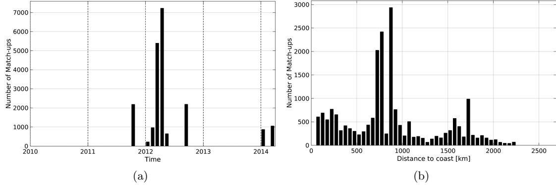
Figure 1: Number of match-ups between TSG-GOSUD-Research-vessel and Aquarius-L4-IPRC-V4-WEEKLY SSS as a function of time (a) and as function of the distance to coast (b) over the North Pacific Ocean Pi-MEP region and for the full satellite product period.
