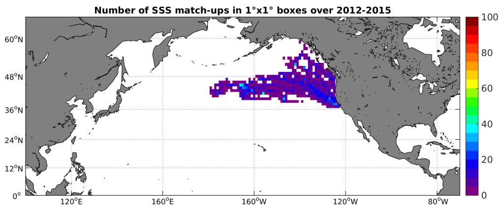
Figure 4: Number of SSS match-ups between Sea mammals SSS and the Aquarius-L4-IPRC-V4-WEEKLY SSS product for the North Pacific Ocean Pi-MEP region over 1°x1° boxes and for the full satellite product period.
