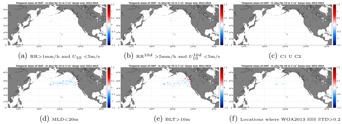
Figure 12: Temporal mean gridded over spatial boxes of size 1^\circ \times 1^\circ of \Delta SSS (Aquarius-L4-IPRC-V4-WEEKLY - Sea mammals) for 6 different subdatasets corresponding to:RR>1mm/h and U_{10} < 5m/s (a), RR^{10d} > 5mm/h and U_{10}^{10d} < 5m/s (b), C1 U C2 (c),MLD<20m (d),BLT>10m (e),Locations where WOA2013 SSS STD>0.2 (f).
