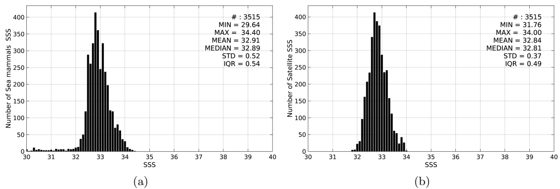
Figure 2: Histograms of SSS from Sea mammals (a) and Aquarius-L4-IPRC-V4-WEEKLY (b) considering all match-up pairs per bins of 0.1 over the North Pacific Ocean Pi-MEP region and for the full satellite product period.
