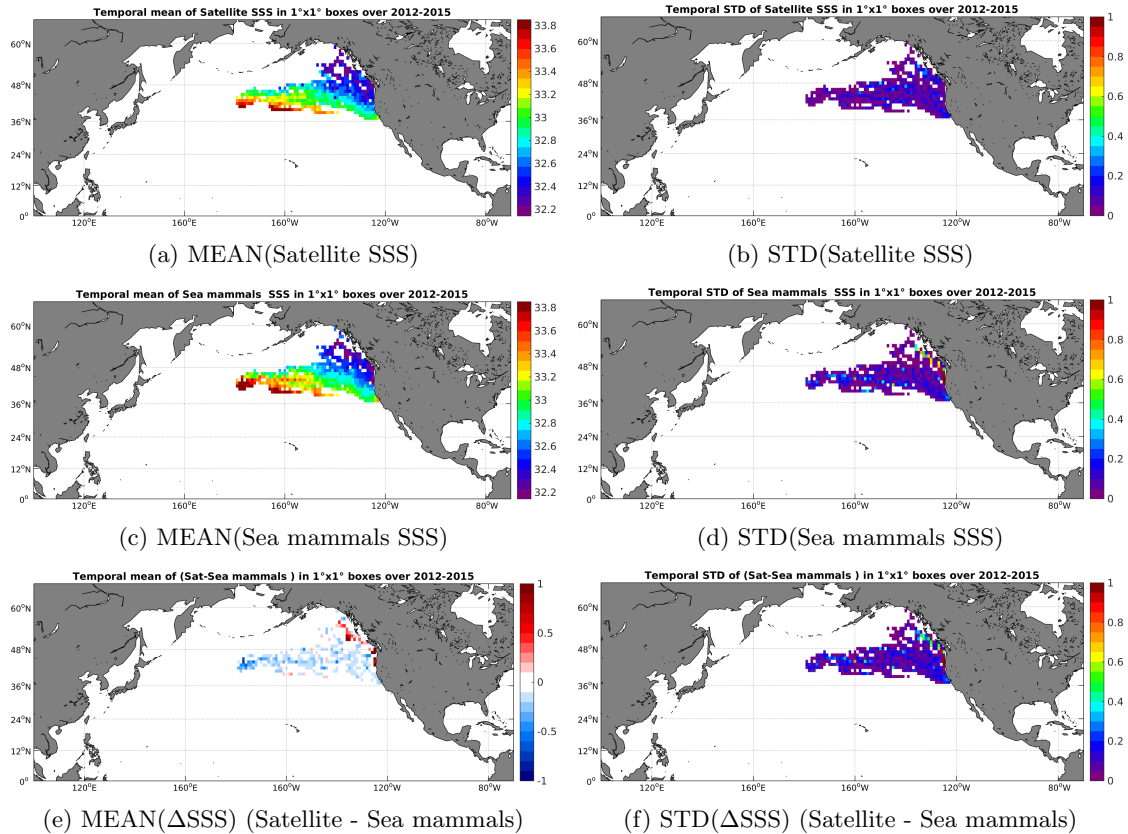
Figure 6: Temporal mean (left) and STD (right) of SSS from Aquarius-L4-IPRC-V4-WEEKLY (top), Sea mammals (middle), and of \Delta SSS (Satellite - Sea mammals). Only match-up pairs are used to generate these maps.
