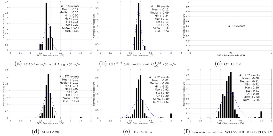
Figure 13: Normalized histogram of \Delta\text{SSS} (Aquarius-L4-IPRC-V4-WEEKLY - Sea mammals) for 6 different subdatasets corresponding to: \text{RR}>1\text{mm/h} and U_{10} <5\text{m/s} (a), \text{RR}^{10d} >5\text{mm/h} and U_{10}^{10d} <5\text{m/s} (b), C1 U C2 (c), \text{MLD}<20\text{m} (d), \text{BLT}>10\text{m} (e), Locations where WOA2013 SSS \text{STD}>0.2 (f).
