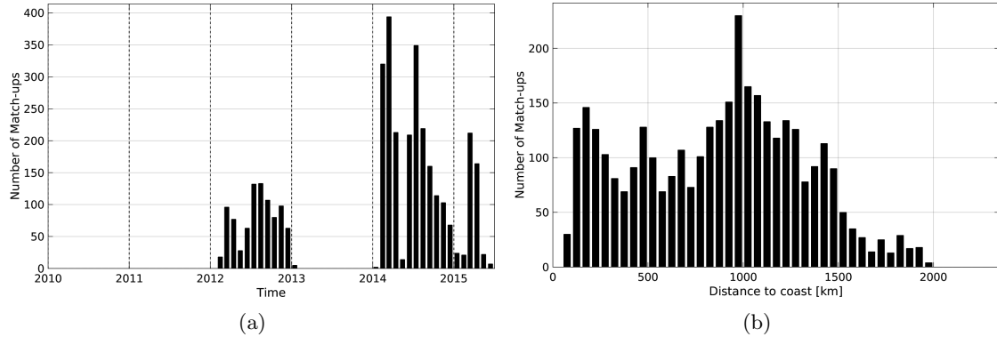
Figure 1: Number of match-ups between Sea mammals and Aquarius-L4-IPRC-V4-WEEKLY SSS as a function of time (a) and as function of the distance to coast (b) over the North Pacific Ocean Pi-MEP region and for the full satellite product period.
