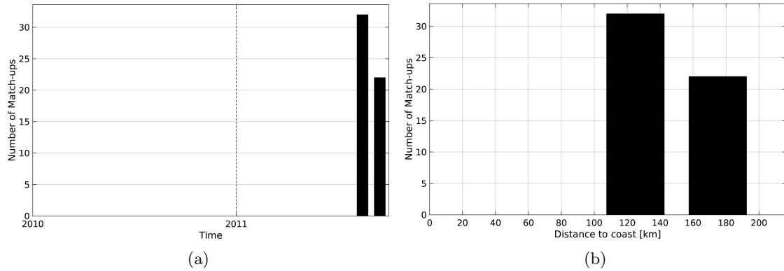
Figure 1: Number of match-ups between Surface drifters and Aquarius-L4-IPRC-V4-WEEKLY SSS as a function of time (a) and as function of the distance to coast (b) over the North Pacific Ocean Pi-MEP region and for the full satellite product period.
