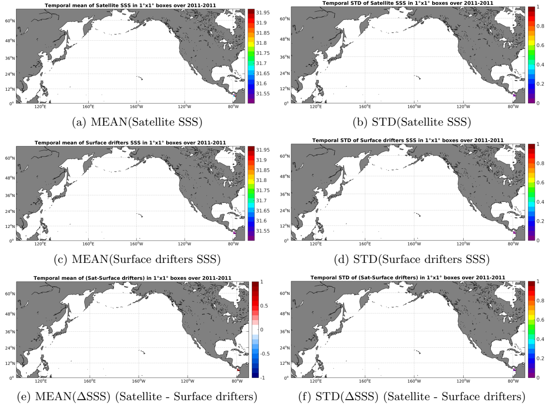
Figure 5: Temporal mean (left) and STD (right) of SSS from Aquarius-L4-IPRC-V4-WEEKLY (top), Surface drifters (middle), and of \Delta SSS (Satellite - Surface drifters). Only match-up pairs are used to generate these maps.
