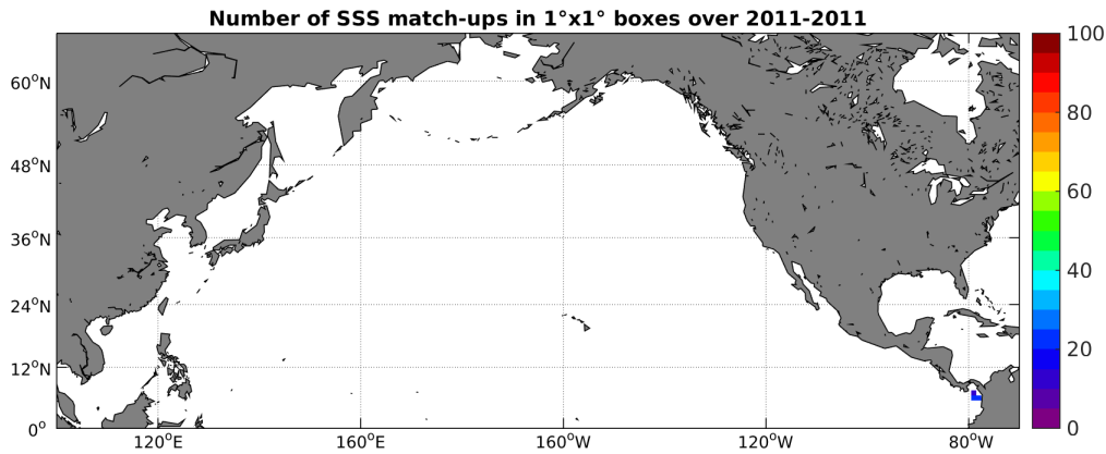
Figure 3: Number of SSS match-ups between Surface drifters SSS and the Aquarius-L4-IPRC-V4-WEEKLY SSS product for the North Pacific Ocean Pi-MEP region over 1^\circ \times 1^\circ boxes and for the full satellite product period.
