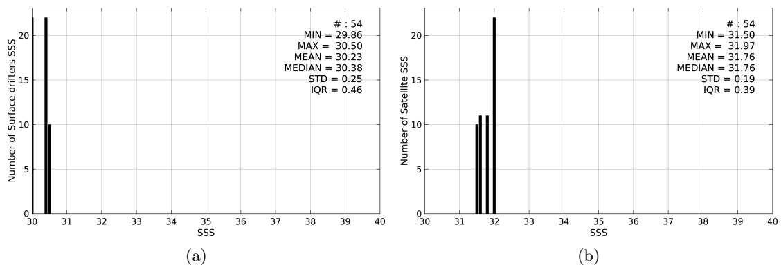
Figure 2: Histograms of SSS from Surface drifters (a) and Aquarius-L4-IPRC-V4-WEEKLY (b) considering all match-up pairs per bins of 0.1 over the North Pacific Ocean Pi-MEP region and for the full satellite product period.
