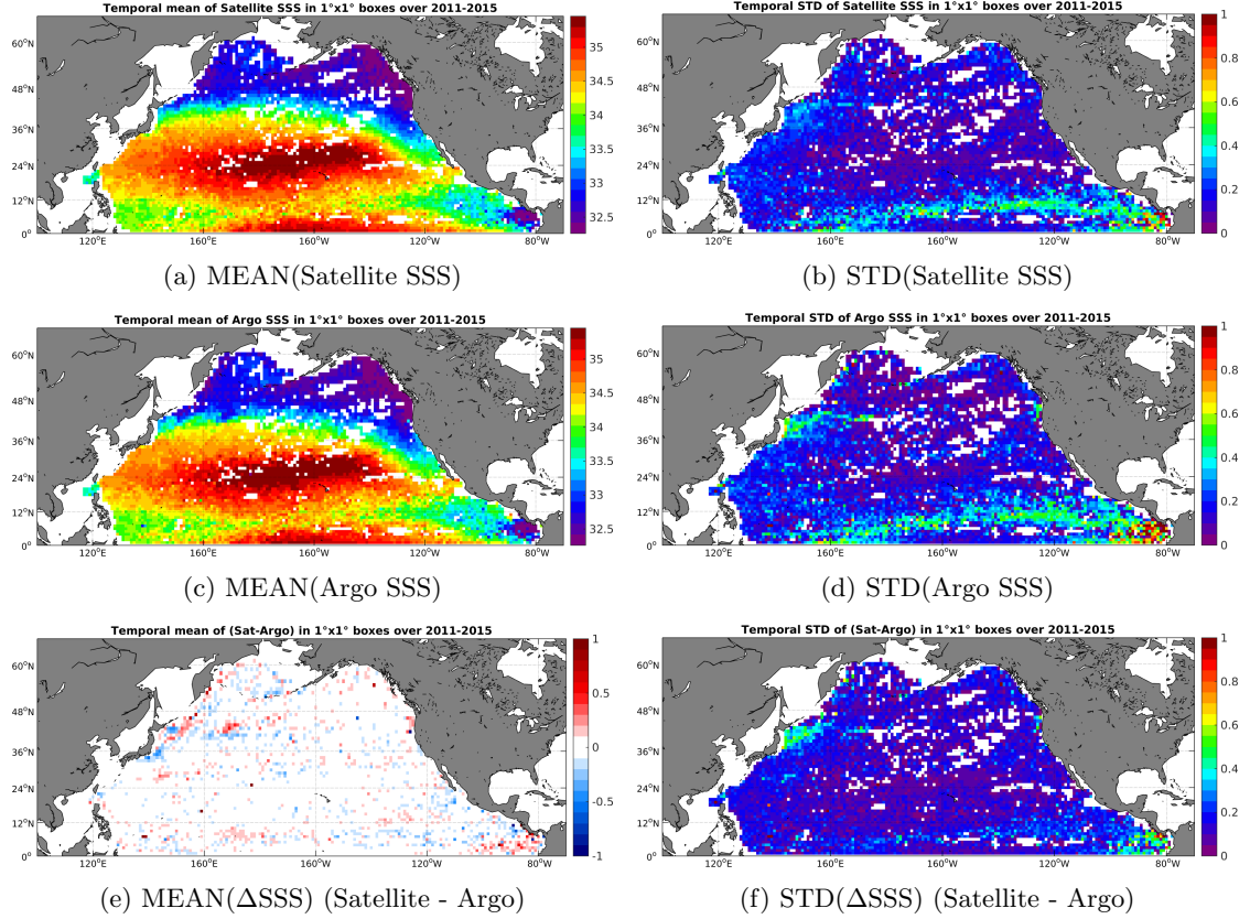
Figure 6: Temporal mean (left) and STD (right) of SSS from Aquarius-L4-IPRC-V4-WEEKLY (top), Argo (middle), and of \Delta SSS (Satellite - Argo). Only match-up pairs are used to generate these maps.
