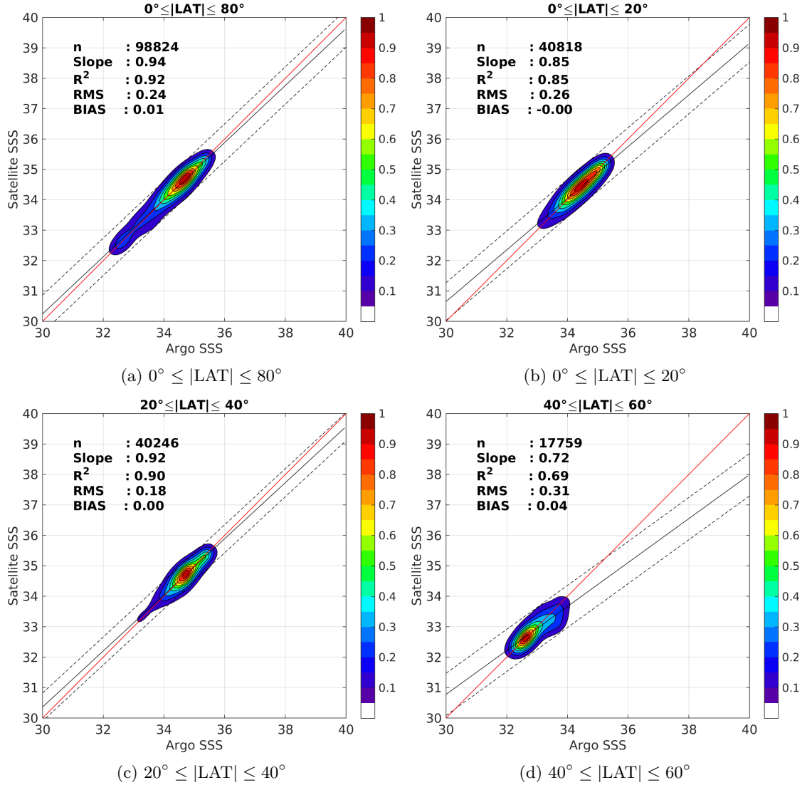
Figure 9: Contour maps of the concentration of Aquarius-L4-IPRC-V4-WEEKLY SSS (y-axis) versus Argo SSS (x-axis) at match-up pairs for different latitude bands. For each plot, the red line shows x=y . The black thin and dashed lines indicate a linear fit through the data cloud and the \pm 95\% confidence levels, respectively. The number match-up pairs n , the slope and R^2 coefficient of the linear fit, the root mean square (RMS) and the mean bias between satellite and in situ data are indicated for each latitude band in each plots.
