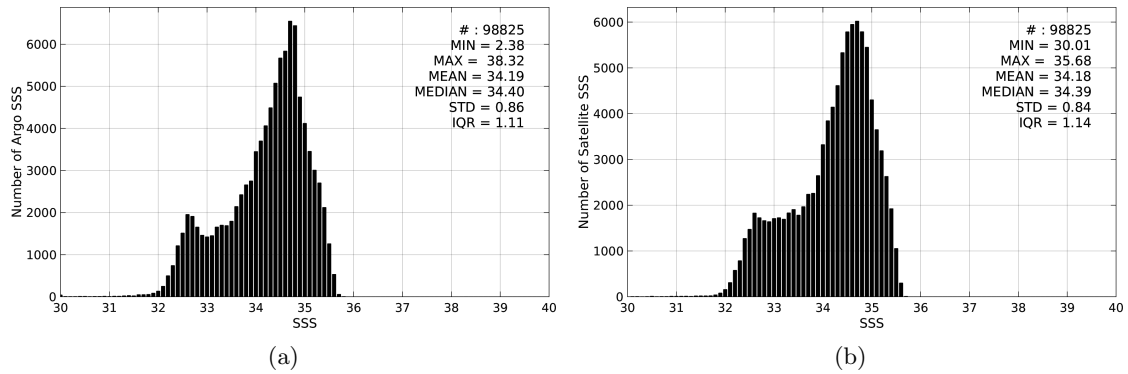
Figure 2: Histograms of SSS from Argo (a) and Aquarius-L4-IPRC-V4-WEEKLY (b) considering all match-up pairs per bins of 0.1 over the North Pacific Ocean Pi-MEP region and for the full satellite product period.
