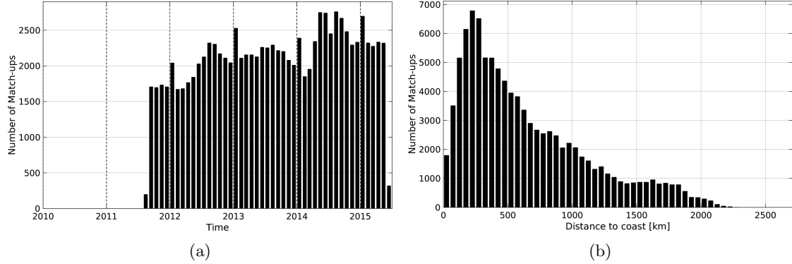
Figure 1: Number of match-ups between Argo and Aquarius-L4-IPRC-V4-WEEKLY SSS as a function of time (a) and as function of the distance to coast (b) over the North Pacific Ocean Pi-MEP region and for the full satellite product period.
