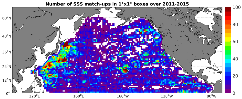
Figure 4: Number of SSS match-ups between Argo SSS and the Aquarius-L4-IPRC-V4-WEEKLY SSS product for the North Pacific Ocean Pi-MEP region over 1^\circ \times 1^\circ boxes and for the full satellite product period.
