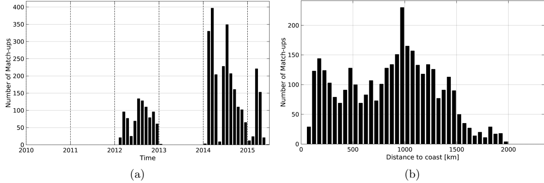
Figure 1: Number of match-ups between Sea mammals and Aquarius-L4-IPRC-V4-MONTHLY SSS as a function of time (a) and as function of the distance to coast (b) over the North Pacific Ocean Pi-MEP region and for the full satellite product period.
