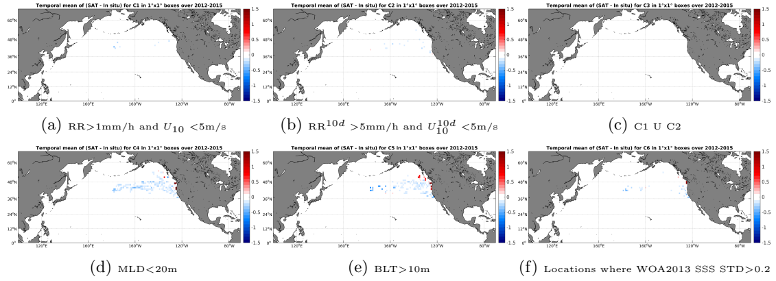
Figure 12: Temporal mean gridded over spatial boxes of size 1^\circ \times 1^\circ of \Delta SSS (Aquarius-L4-IPRC-V4-MONTHLY - Sea mammals) for 6 different subdatasets corresponding to: RR > 1\text{mm/h} and U_{10} < 5\text{m/s} (a), RR^{10d} > 5\text{mm/h} and U_{10}^{10d} < 5\text{m/s} (b), C1 U C2 (c), MLD < 20\text{m} (d), BLT > 10\text{m} (e), Locations where WOA2013 SSS STD > 0.2 (f).
