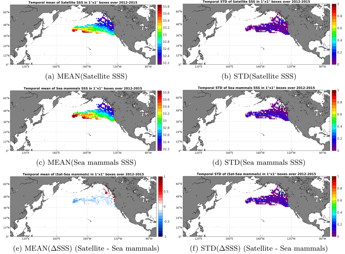
Figure 6: Temporal mean (left) and STD (right) of SSS from Aquarius-L4-IPRC-V4-MONTHLY (top), Sea mammals (middle), and of \Delta SSS (Satellite - Sea mammals). Only match-up pairs are used to generate these maps.
