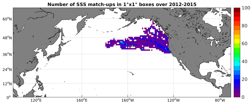
Figure 4: Number of SSS match-ups between Sea mammals SSS and the Aquarius-L4-IPRC-V4-MONTHLY SSS product for the North Pacific Ocean Pi-MEP region over 1^\circ \times 1^\circ boxes and for the full satellite product period.
