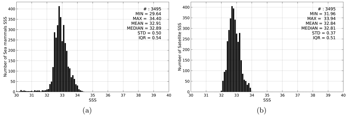
Figure 2: Histograms of SSS from Sea mammals (a) and Aquarius-L4-IPRC-V4-MONTHLY (b) considering all match-up pairs per bins of 0.1 over the North Pacific Ocean Pi-MEP region and for the full satellite product period.
