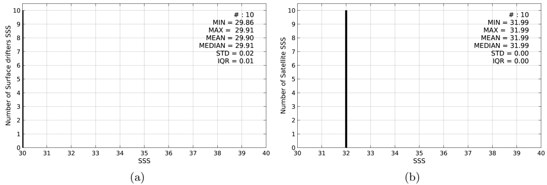
Figure 2: Histograms of SSS from Surface drifters (a) and Aquarius-L4-IPRC-V4-MONTHLY (b) considering all match-up pairs per bins of 0.1 over the North Pacific Ocean Pi-MEP region and for the full satellite product period.
