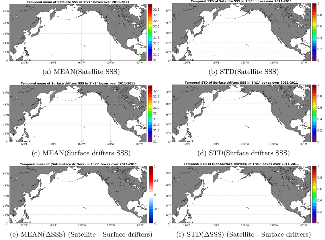
Figure 5: Temporal mean (left) and STD (right) of SSS from Aquarius-L4-IPRC-V4-MONTHLY (top), Surface drifters (middle), and of \Delta SSS (Satellite - Surface drifters). Only match-up pairs are used to generate these maps.
