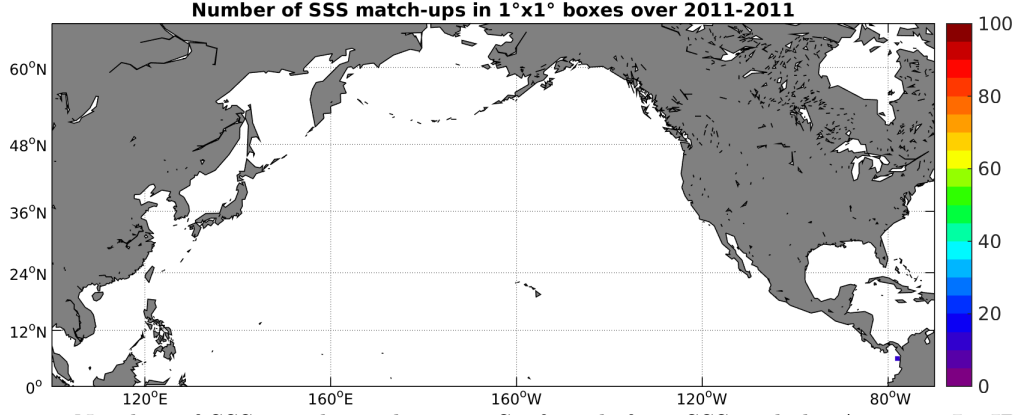
Figure 3: Number of SSS match-ups between Surface drifters SSS and the Aquarius-L4-IPRC-V4-MONTHLY SSS product for the North Pacific Ocean Pi-MEP region over 1^\circ \times 1^\circ boxes and for the full satellite product period.
