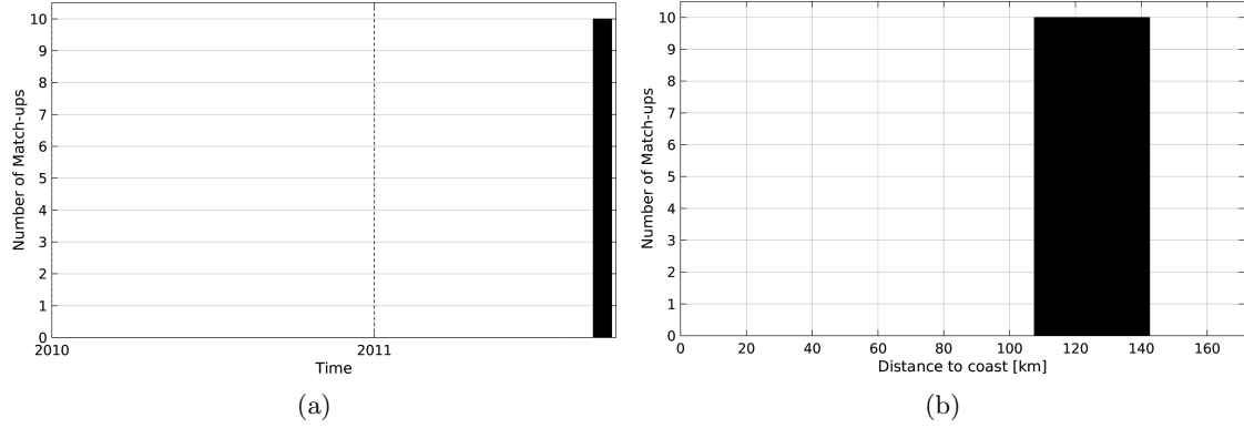
Figure 1: Number of match-ups between Surface drifters and Aquarius-L4-IPRC-V4-MONTHLY SSS as a function of time (a) and as function of the distance to coast (b) over the North Pacific Ocean Pi-MEP region and for the full satellite product period.
