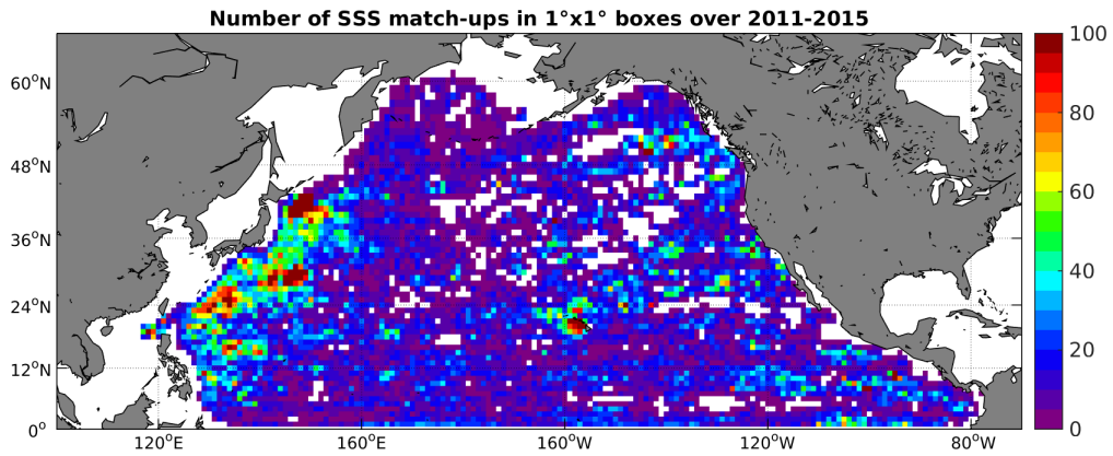
Figure 4: Number of SSS match-ups between Argo SSS and the Aquarius-L4-IPRC-V4-MONTHLY SSS product for the North Pacific Ocean Pi-MEP region over 1°x1° boxes and for the full satellite product period.
