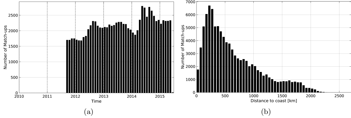
Figure 1: Number of match-ups between Argo and Aquarius-L4-IPRC-V4-MONTHLY SSS as a function of time (a) and as function of the distance to coast (b) over the North Pacific Ocean Pi-MEP region and for the full satellite product period.
