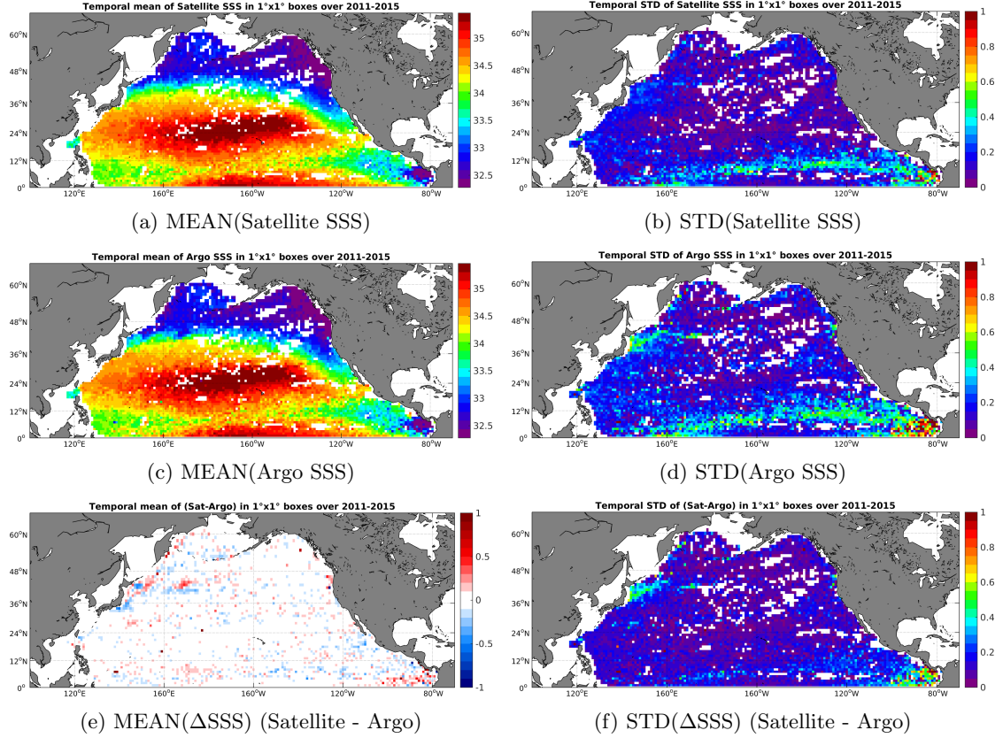
Figure 6: Temporal mean (left) and STD (right) of SSS from Aquarius-L4-IPRC-V4-MONTHLY (top), Argo (middle), and of \Delta SSS (Satellite - Argo). Only match-up pairs are used to generate these maps.
