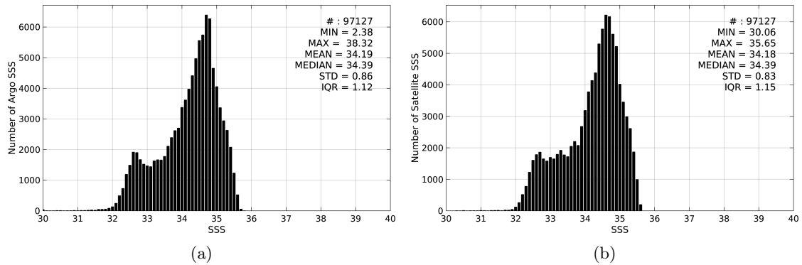
Figure 2: Histograms of SSS from Argo (a) and Aquarius-L4-IPRC-V4-MONTHLY (b) considering all match-up pairs per bins of 0.1 over the North Pacific Ocean Pi-MEP region and for the full satellite product period.
