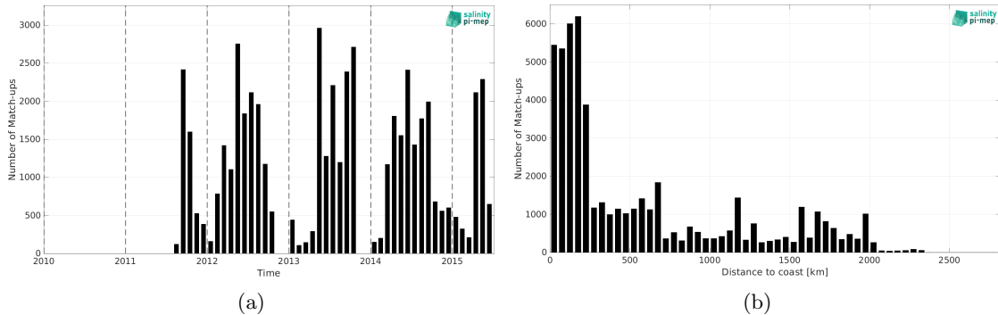
Figure 2: Number of match-ups between TSG (SAMOS) and Aquarius SSS L3 OR v5 - 7-Day running (NASA-GSFC) SSS as a function of time (a) and as function of the distance to coast (b) over the North Pacific Ocean Pi-MEP region and for the full satellite product period.
