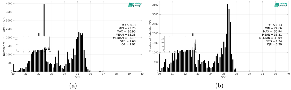
Figure 3: Histograms of SSS from TSG (SAMOS) (a) and Aquarius SSS L3 OR v5 - 7-Day running (NASA-GSFC) (b) considering all match-up pairs per bins of 0.1 over the North Pacific Ocean Pi-MEP region and for the full satellite product period.
