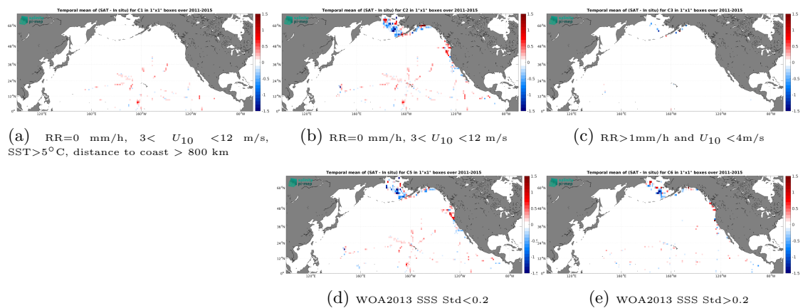
Figure 14: Temporal mean gridded over spatial boxes of size 1^\circ \times 1^\circ of \Delta SSS (Aquarius SSS L3 OR v5 - 7-Day running (NASA-GSFC) - TSG (SAMOS)) for 5 different subdatasets corresponding to:RR=0 mm/h, 3 < U_{10} < 12 m/s, SST >5^\circ\text{C} , distance to coast > 800 km (a), RR=0 mm/h, 3 < U_{10} < 12 m/s (b), RR >1 mm/h and U_{10} < 4 m/s (c), WOA2013 SSS Std <0.2 (d), WOA2013 SSS Std >0.2 (e).
