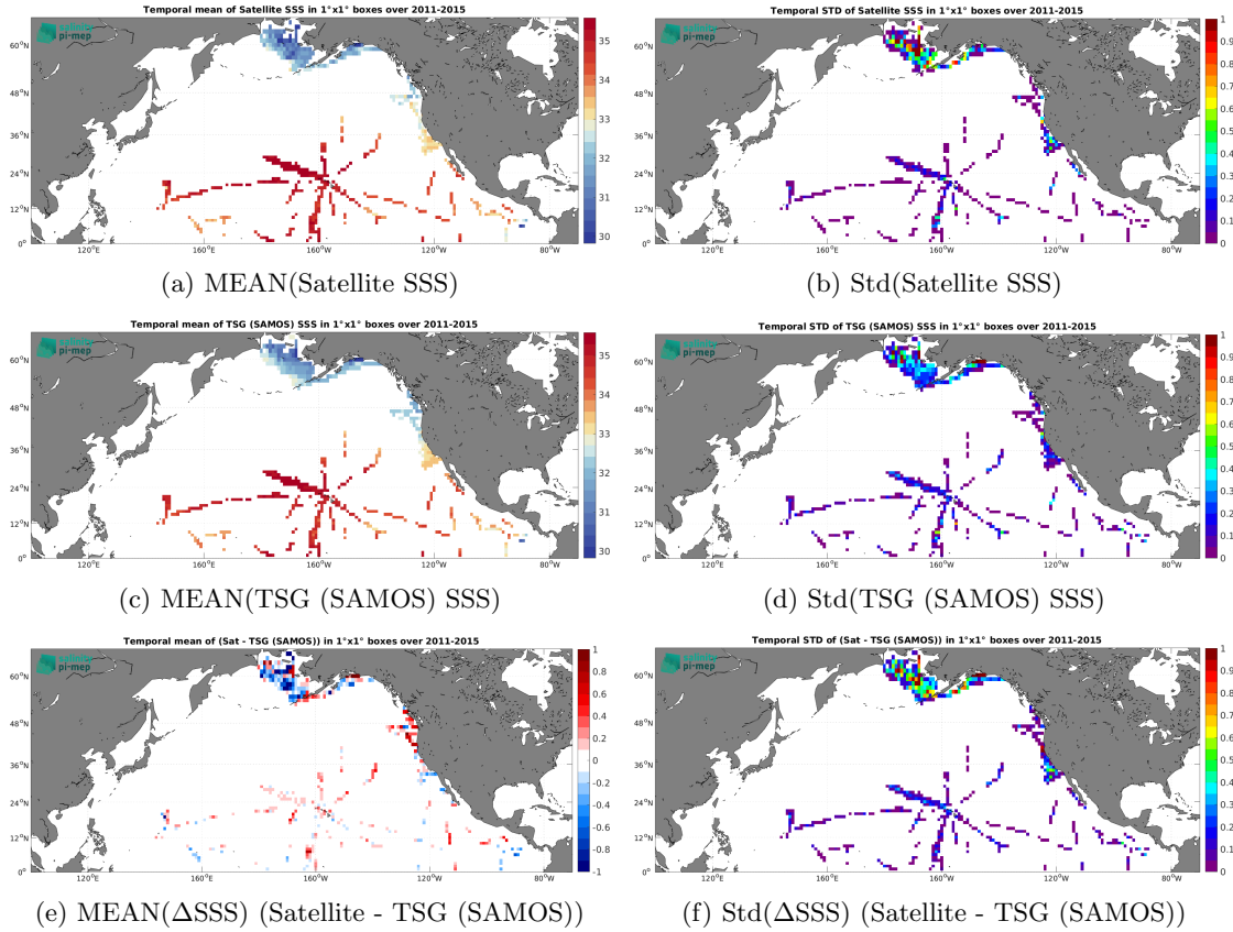
Figure 7: Temporal mean (left) and Std (right) of SSS from Aquarius SSS L3 OR v5 - 7-Day running (NASA-GSFC) (top), TSG (SAMOS) (middle), and of \Delta SSS (Satellite - TSG (SAMOS)). Only match-up pairs are used to generate these maps.
