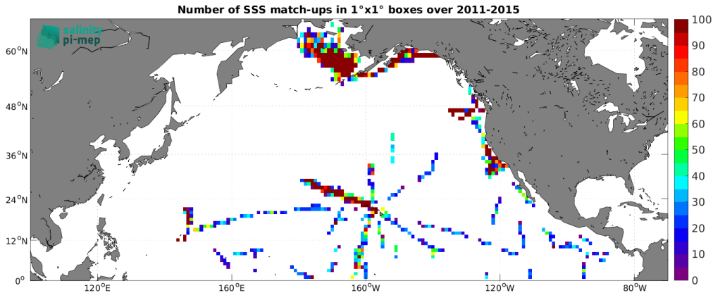
Figure 5: Number of SSS match-ups between TSG (SAMOS) SSS and the Aquarius SSS L3 OR v5 - 7-Day running (NASA-GSFC) SSS product for the North Pacific Ocean Pi-MEP region over 1^\circ \times 1^\circ boxes and for the full satellite product period.
