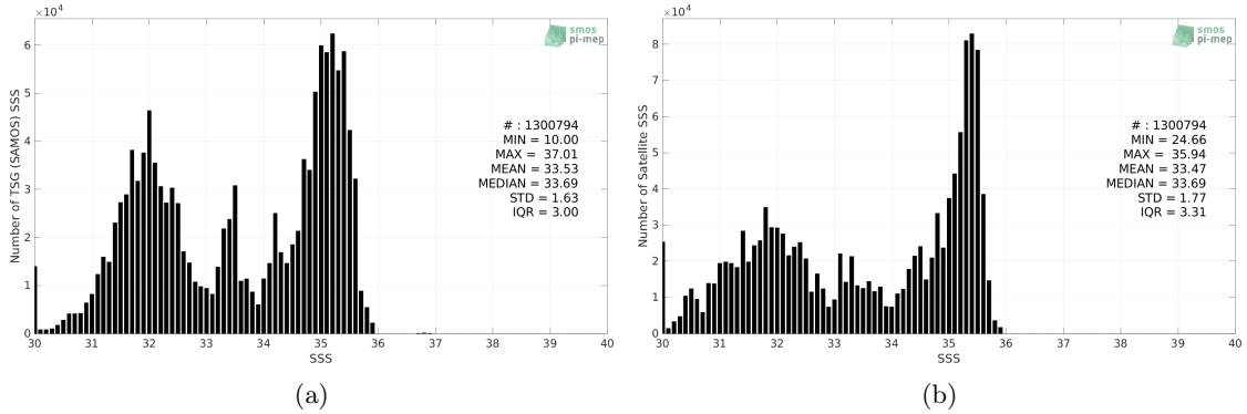
Figure 2: Histograms of SSS from TSG (SAMOS) (a) and Aquarius SSS L3 OR v5 - 7-Day running (NASA-GSFC) (b) considering all match-up pairs per bins of 0.1 over the North Pacific Ocean Pi-MEP region and for the full satellite product period.
