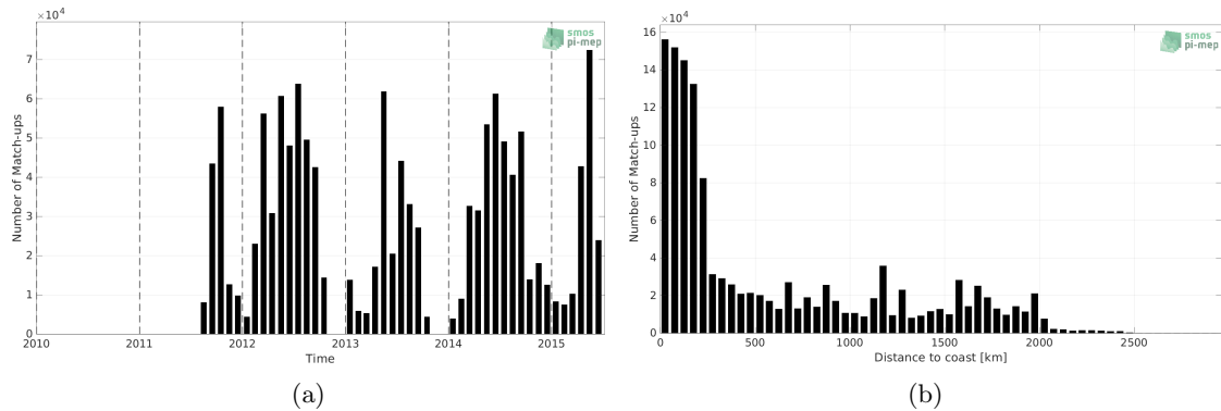
Figure 1: Number of match-ups between TSG (SAMOS) and Aquarius SSS L3 OR v5 - 7-Day running (NASA-GSFC) SSS as a function of time (a) and as function of the distance to coast (b) over the North Pacific Ocean Pi-MEP region and for the full satellite product period.
