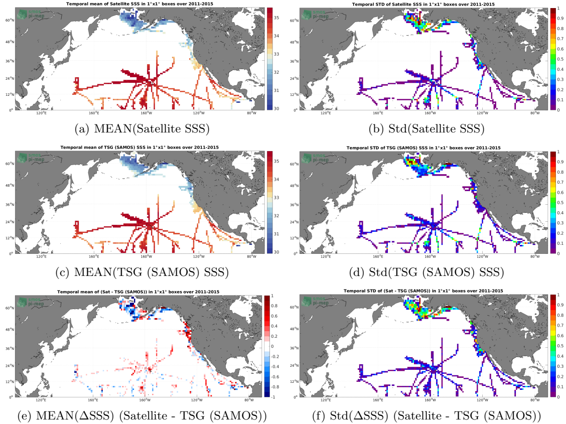
Figure 6: Temporal mean (left) and Std (right) of SSS from Aquarius SSS L3 OR v5 - 7-Day running (NASA-GSFC) (top), TSG (SAMOS) (middle), and of \Delta\text{SSS} (Satellite - TSG (SAMOS)). Only match-up pairs are used to generate these maps.
