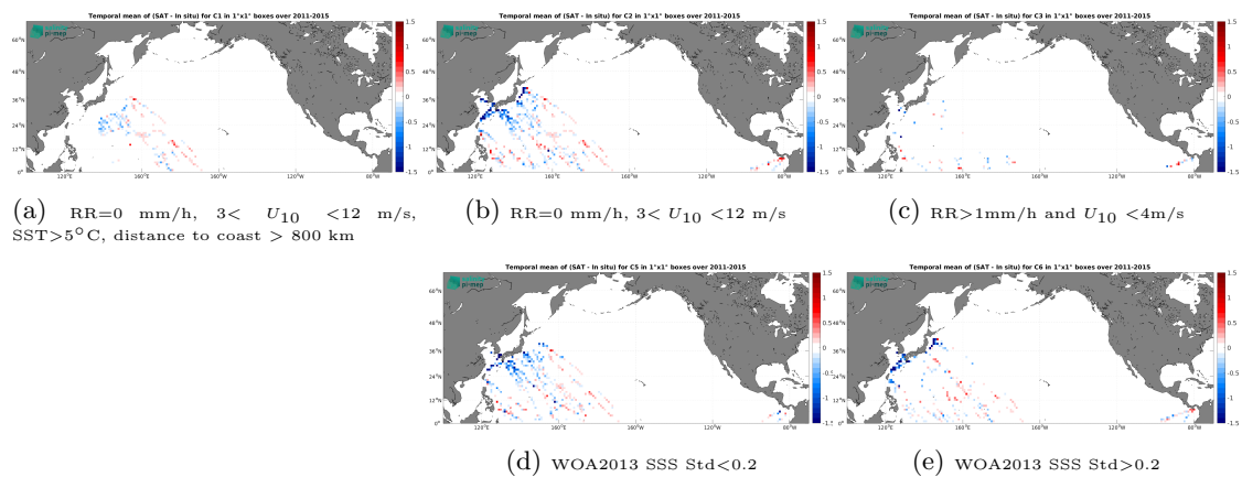
Figure 14: Temporal mean gridded over spatial boxes of size 1^\circ \times 1^\circ of \Delta\text{SSS} (Aquarius SSS L3 OR v5 - 7-Day running (NASA-GSFC) - TSG (LEGOS-DM)) for 5 different subdatasets corresponding to:RR=0 mm/h, 3 < U_{10} < 12 m/s, SST >5^\circ\text{C} , distance to coast > 800 km (a), RR=0 mm/h, 3 < U_{10} < 12 m/s (b), RR >1 mm/h and U_{10} < 4 m/s (c), WOA2013 SSS Std <0.2 (d), WOA2013 SSS Std >0.2 (e).
