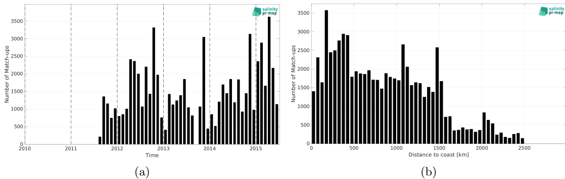
Figure 2: Number of match-ups between TSG (LEGOS-DM) and Aquarius SSS L3 OR v5 - 7-Day running (NASA-GSFC) SSS as a function of time (a) and as function of the distance to coast (b) over the North Pacific Ocean Pi-MEP region and for the full satellite product period.
