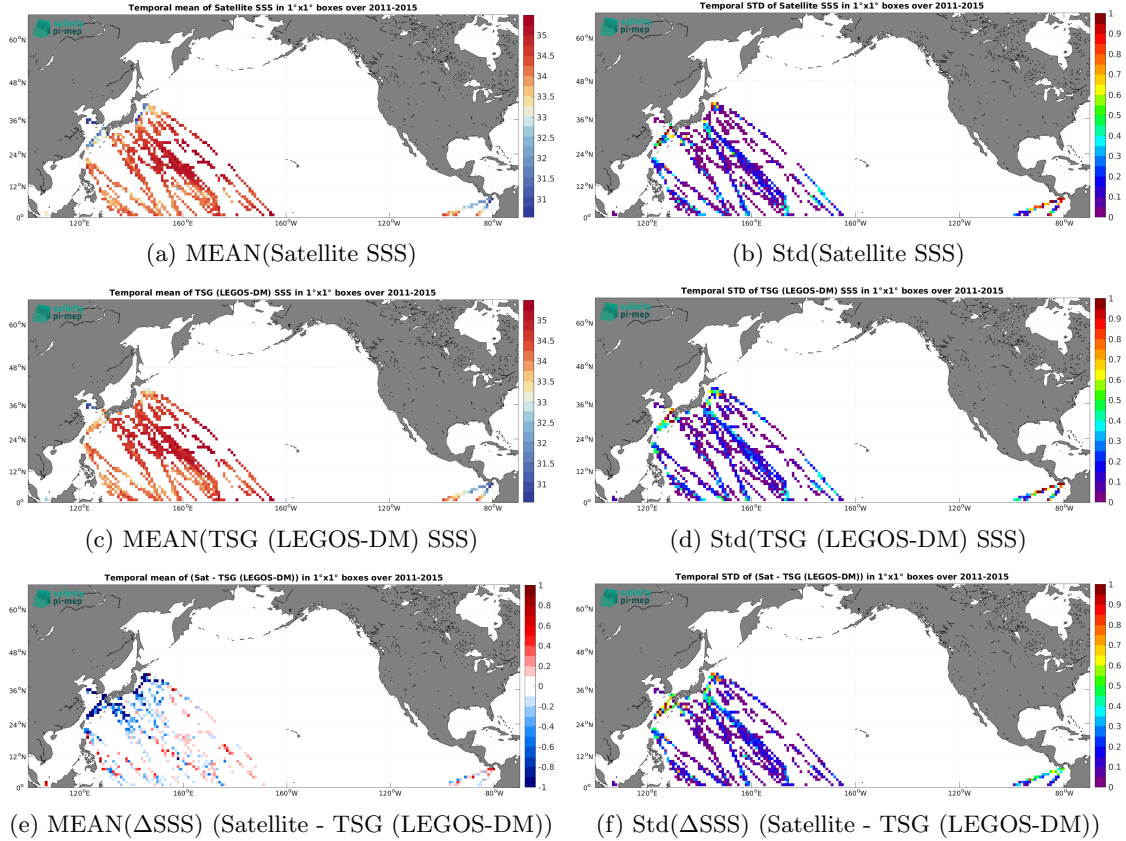
Figure 7: Temporal mean (left) and Std (right) of SSS from Aquarius SSS L3 OR v5 - 7-Day running (NASA-GSFC) (top), TSG (LEGOS-DM) (middle), and of \Delta SSS (Satellite - TSG (LEGOS-DM)). Only match-up pairs are used to generate these maps.
