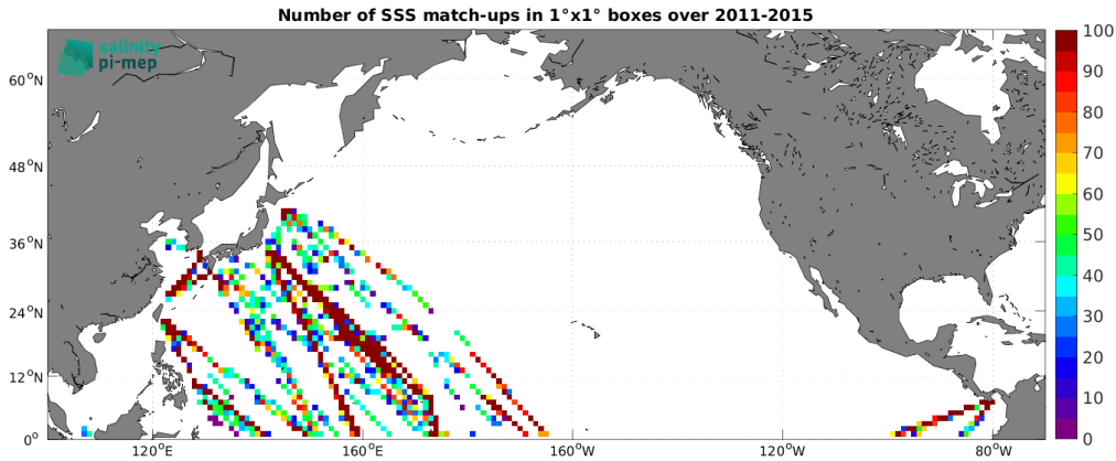
Figure 5: Number of SSS match-ups between TSG (LEGOS-DM) SSS and the Aquarius SSS L3 OR v5 - 7-Day running (NASA-GSFC) SSS product for the North Pacific Ocean Pi-MEP region over 1^\circ \times 1^\circ boxes and for the full satellite product period.
