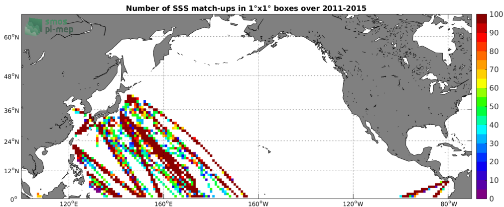
Figure 4: Number of SSS match-ups between TSG-LEGOS-DM SSS and the Aquarius-L3-OR-V5-7DAY-RUNNING-1DEG SSS product for the North Pacific Ocean Pi-MEP region over 1^\circ \times 1^\circ boxes and for the full satellite product period.
