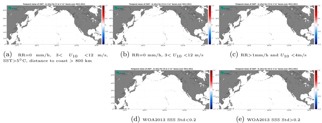
Figure 14: Temporal mean gridded over spatial boxes of size 1^\circ \times 1^\circ of \Delta\text{SSS} (Aquarius SSS L3 OR v5 - 7-Day running (NASA-GSFC) - TSG (GOSUD-Sailing-ship)) for 5 different subdatasets corresponding to:RR=0 mm/h, 3 < U_{10} < 12 m/s, SST >5^\circ\text{C} , distance to coast > 800 km (a), RR=0 mm/h, 3 < U_{10} < 12 m/s (b), RR >1 mm/h and U_{10} < 4 m/s (c), WOA2013 SSS Std <0.2 (d), WOA2013 SSS Std >0.2 (e).
