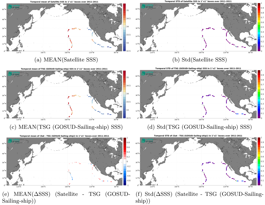
Figure 7: Temporal mean (left) and Std (right) of SSS from Aquarius SSS L3 OR v5 - 7-Day running (NASA-GSFC) (top), TSG (GOSUD-Sailing-ship) (middle), and of \Delta SSS (Satellite - TSG (GOSUD-Sailing-ship)). Only match-up pairs are used to generate these maps.
