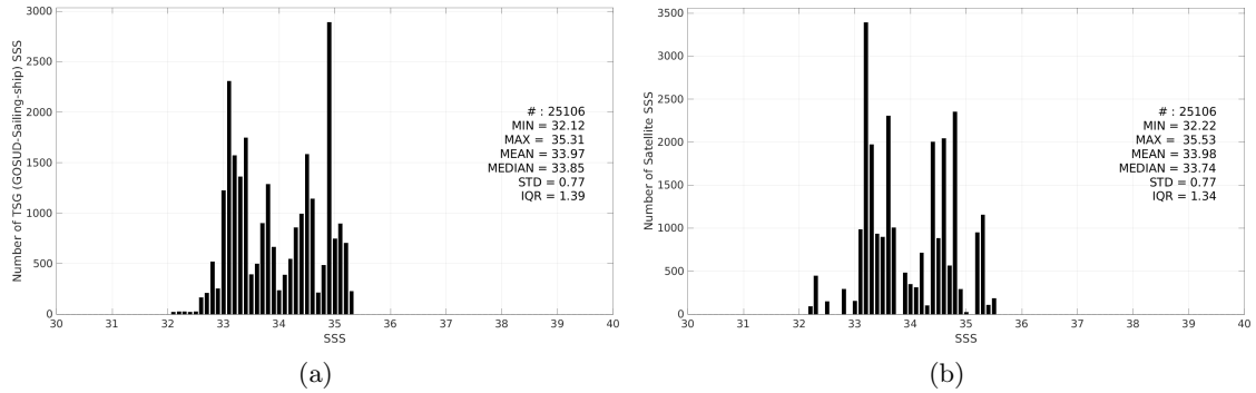
Figure 3: Histograms of SSS from TSG (GOSUD-Sailing-ship) (a) and Aquarius SSS L3 OR v5 - 7-Day running (NASA-GSFC) (b) considering all match-up pairs per bins of 0.1 over the North Pacific Ocean Pi-MEP region and for the full satellite product period.
