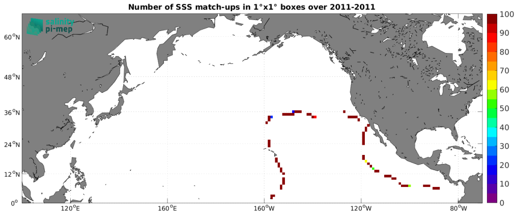
Figure 5: Number of SSS match-ups between TSG (GOSUD-Sailing-ship) SSS and the Aquarius SSS L3 OR v5 - 7-Day running (NASA-GSFC) SSS product for the North Pacific Ocean Pi-MEP region over 1^\circ \times 1^\circ boxes and for the full satellite product period.
