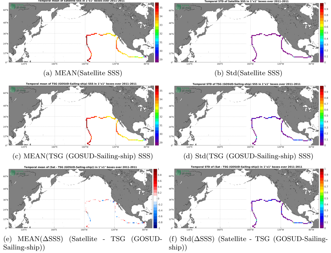
Figure 6: Temporal mean (left) and Std (right) of SSS from Aquarius SSS L3 OR v5 - 7-Day running (NASA-GSFC) (top), TSG (GOSUD-Sailing-ship) (middle), and of \Delta SSS (Satellite - TSG (GOSUD-Sailing-ship)). Only match-up pairs are used to generate these maps.
