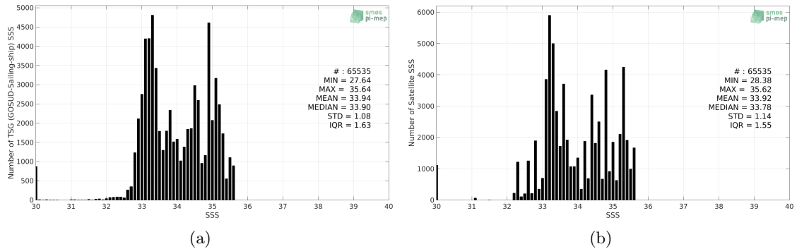
Figure 2: Histograms of SSS from TSG (GOSUD-Sailing-ship) (a) and Aquarius SSS L3 OR v5 - 7-Day running (NASA-GSFC) (b) considering all match-up pairs per bins of 0.1 over the North Pacific Ocean Pi-MEP region and for the full satellite product period.
