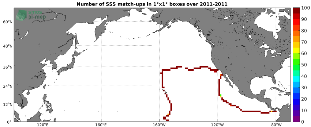
Figure 4: Number of SSS match-ups between TSG (GOSUD-Sailing-ship) SSS and the Aquarius SSS L3 OR v5 - 7-Day running (NASA-GSFC) SSS product for the North Pacific Ocean Pi-MEP region over 1^\circ \times 1^\circ boxes and for the full satellite product period.
