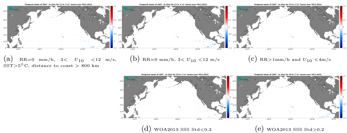
Figure 14: Temporal mean gridded over spatial boxes of size 1^\circ \times 1^\circ of \Delta\text{SSS} (Aquarius SSS L3 OR v5 - 7-Day running (NASA-GSFC) - TSG (GOSUD-Research-vessel)) for 5 different subdatasets corresponding to:RR=0 mm/h, 3 < U_{10} < 12 m/s, SST >5^\circ\text{C} , distance to coast > 800 km (a), RR=0 mm/h, 3 < U_{10} < 12 m/s (b), RR >1 mm/h and U_{10} < 4 m/s (c), WOA2013 SSS Std <0.2 (d), WOA2013 SSS Std >0.2 (e).
