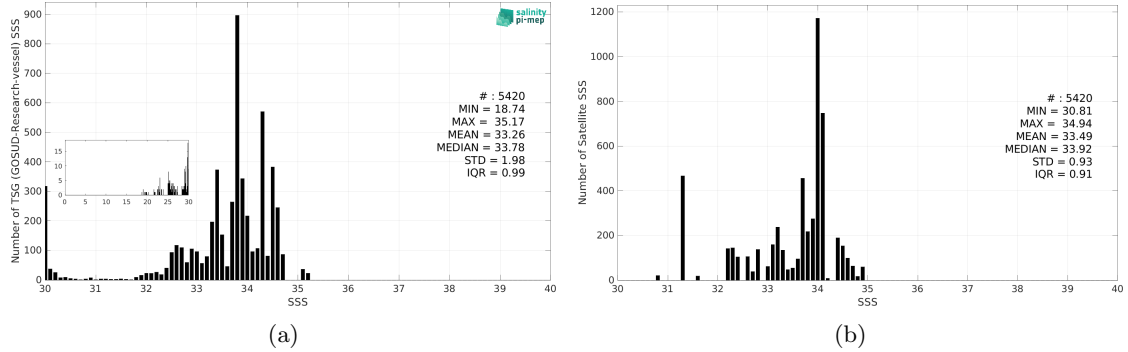
Figure 3: Histograms of SSS from TSG (GOSUD-Research-vessel) (a) and Aquarius SSS L3 OR v5 - 7-Day running (NASA-GSFC) (b) considering all match-up pairs per bins of 0.1 over the North Pacific Ocean Pi-MEP region and for the full satellite product period.
