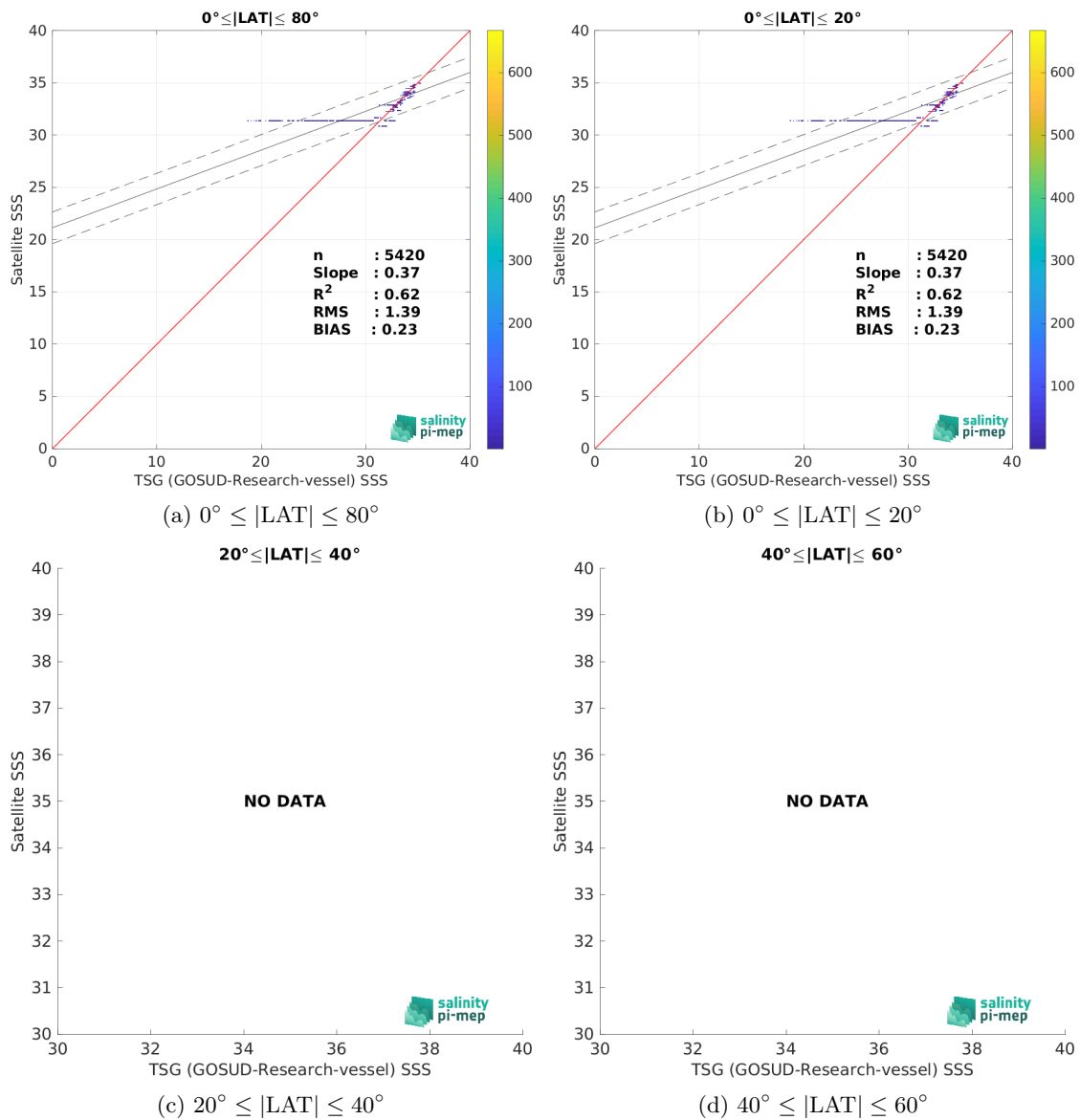
Figure 10: Contour maps of the concentration of Aquarius SSS L3 OR v5 - 7-Day running (NASA-GSFC) SSS ( y -axis) versus TSG (GOSUD-Research-vessel) SSS ( x -axis) at match-up pairs for different latitude bands. For each plot, the red line shows x=y . The black thin and dashed lines indicate a linear fit through the data cloud and the \pm 95\% confidence levels, respectively. The number match-up pairs n , the slope and R^2 coefficient of the linear fit, the root mean square (RMS) and the mean bias between satellite and in situ data are indicated for each latitude band in each plots.
