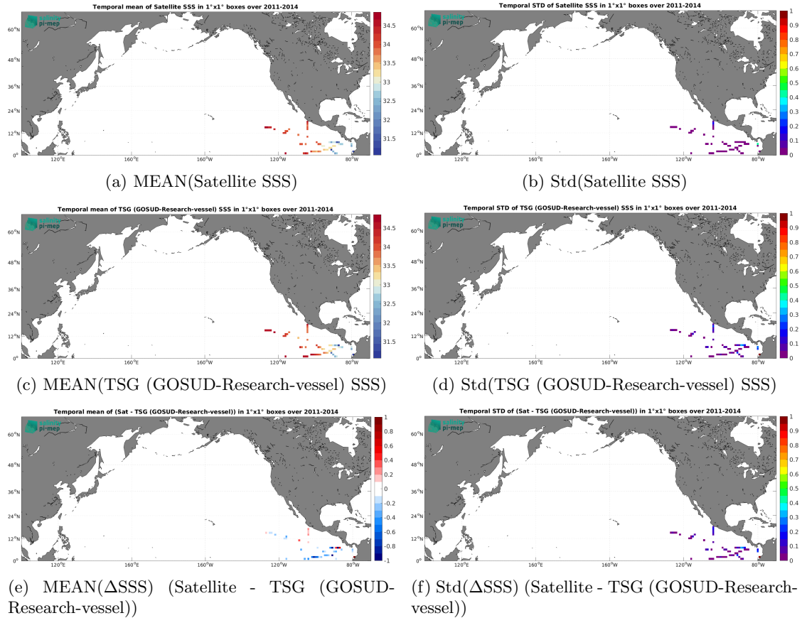
Figure 7: Temporal mean (left) and Std (right) of SSS from Aquarius SSS L3 OR v5 - 7-Day running (NASA-GSFC) (top), TSG (GOSUD-Research-vessel) (middle), and of \Delta\text{SSS} (Satellite - TSG (GOSUD-Research-vessel)). Only match-up pairs are used to generate these maps.
