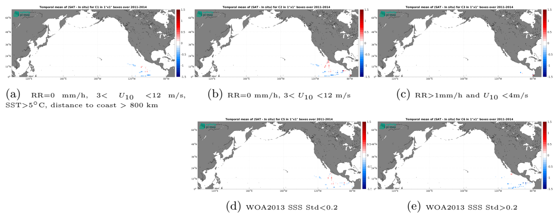
Figure 12: Temporal mean gridded over spatial boxes of size 1^\circ \times 1^\circ of \Delta\text{SSS} (Aquarius SSS L3 OR v5 - 7-Day running (NASA-GSFC) - TSG (GOSUD-Research-vessel)) for 5 different subdatasets corresponding to:RR=0 mm/h, 3 < U_{10} < 12 m/s, SST >5^\circ\text{C} , distance to coast > 800 km (a), RR=0 mm/h, 3 < U_{10} < 12 m/s (b), RR >1 mm/h and U_{10} < 4 m/s (c), WOA2013 SSS Std <0.2 (d), WOA2013 SSS Std >0.2 (e).
