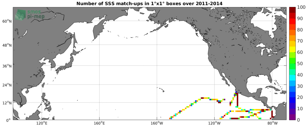
Figure 4: Number of SSS match-ups between TSG-GOSUD-Research-vessel SSS and the Aquarius-L3-OR-V5-7DAY-RUNNING-1DEG SSS product for the North Pacific Ocean Pi-MEP region over 1°x1° boxes and for the full satellite product period.
