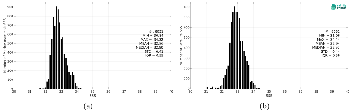
Figure 2: Histograms of SSS from Marine mammals (a) and Aquarius SSS L3 OR v5 - 7-Day running (NASA-GSFC) (b) considering all match-up pairs per bins of 0.1 over the North Pacific Ocean Pi-MEP region and for the full satellite product period.
