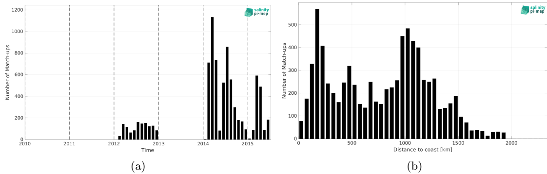
Figure 1: Number of match-ups between Marine mammals and Aquarius SSS L3 OR v5 - 7-Day running (NASA-GSFC) SSS as a function of time (a) and as function of the distance to coast (b) over the North Pacific Ocean Pi-MEP region and for the full satellite product period.
