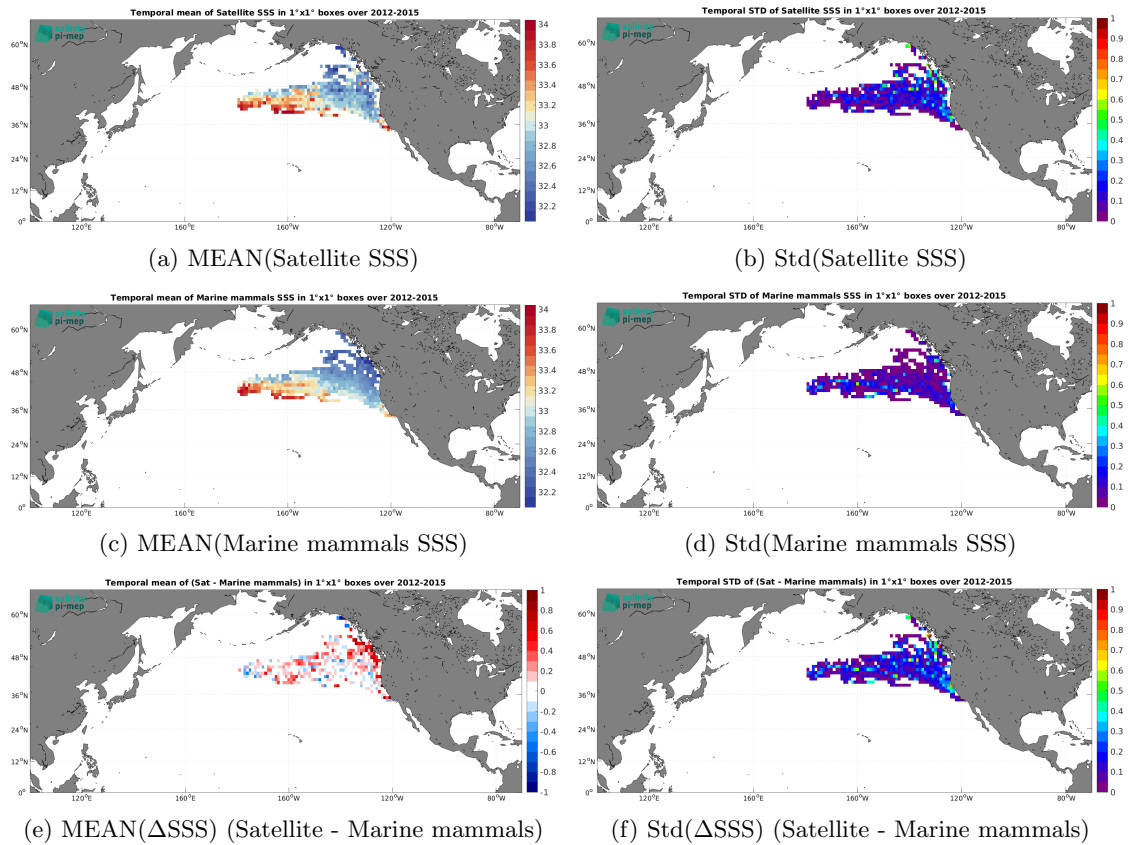
Figure 6: Temporal mean (left) and Std (right) of SSS from Aquarius SSS L3 OR v5 - 7-Day running (NASA-GSFC) (top), Marine mammals (middle), and of \Delta SSS (Satellite - Marine mammals). Only match-up pairs are used to generate these maps.
