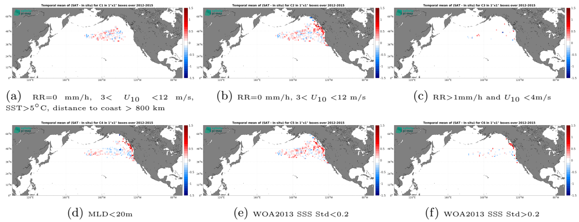
Figure 12: Temporal mean gridded over spatial boxes of size 1^\circ \times 1^\circ of \Delta SSS (Aquarius SSS L3 OR v5 - 7-Day running (NASA-GSFC) - Marine mammals) for 6 different subdatasets corresponding to:RR=0 mm/h, 3 < U_{10} < 12 m/s, SST >5^\circ C, distance to coast > 800 km (a), RR=0 mm/h, 3 < U_{10} < 12 m/s (b), RR >1 mm/h and U_{10} < 4 m/s (c),MLD <20 m (d),WOA2013 SSS Std <0.2 (e),WOA2013 SSS Std >0.2 (f).
