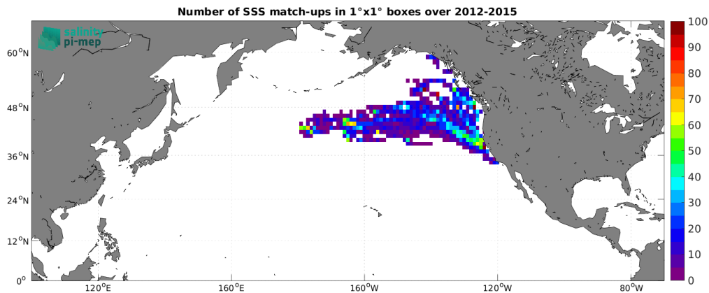
Figure 4: Number of SSS match-ups between Marine mammals SSS and the Aquarius SSS L3 OR v5 - 7-Day running (NASA-GSFC) SSS product for the North Pacific Ocean Pi-MEP region over 1^\circ \times 1^\circ boxes and for the full satellite product period.
