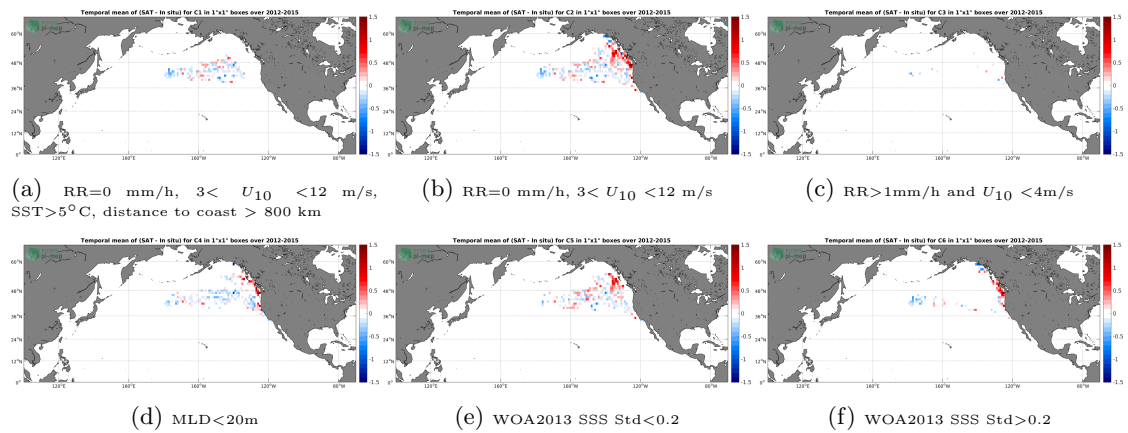
Figure 12: Temporal mean gridded over spatial boxes of size 1^\circ \times 1^\circ of \Delta SSS (Aquarius-L3-OR-V5-7DAY-RUNNING-1DEG - Sea mammals) for 6 different subdatasets corresponding to:RR=0 mm/h, 3 < U_{10} < 12 m/s, SST >5^\circ C, distance to coast > 800 km (a), RR=0 mm/h, 3 < U_{10} < 12 m/s (b), RR >1 mm/h and U_{10} < 4 m/s (c),MLD <20 m (d),WOA2013 SSS Std <0.2 (e),WOA2013 SSS Std >0.2 (f).
