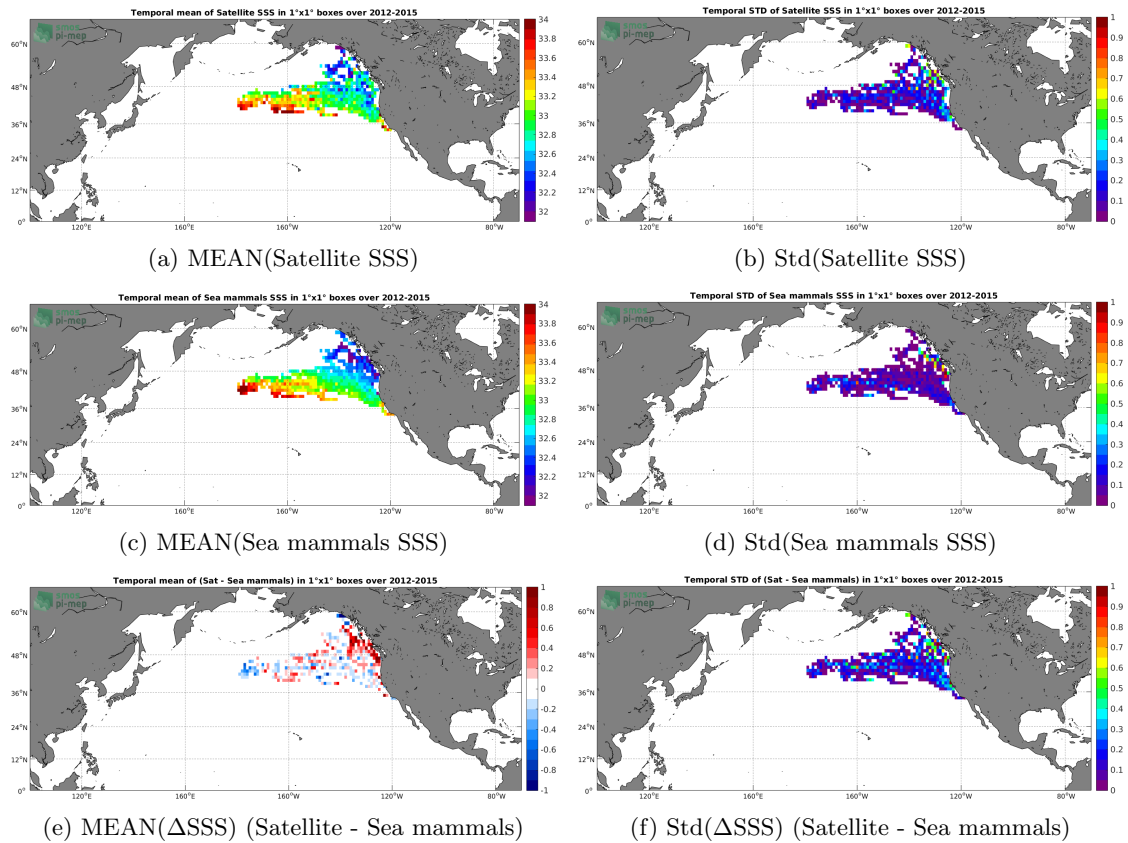
Figure 6: Temporal mean (left) and Std (right) of SSS from Aquarius-L3-OR-V5-7DAY-RUNNING-1DEG (top), Sea mammals (middle), and of \Delta SSS (Satellite - Sea mammals). Only match-up pairs are used to generate these maps.
