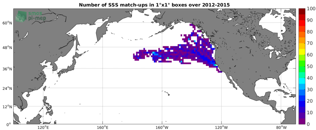
Figure 4: Number of SSS match-ups between Sea mammals SSS and the Aquarius-L3-OR-V5-7DAY-RUNNING-1DEG SSS product for the North Pacific Ocean Pi-MEP region over 1°x1° boxes and for the full satellite product period.
