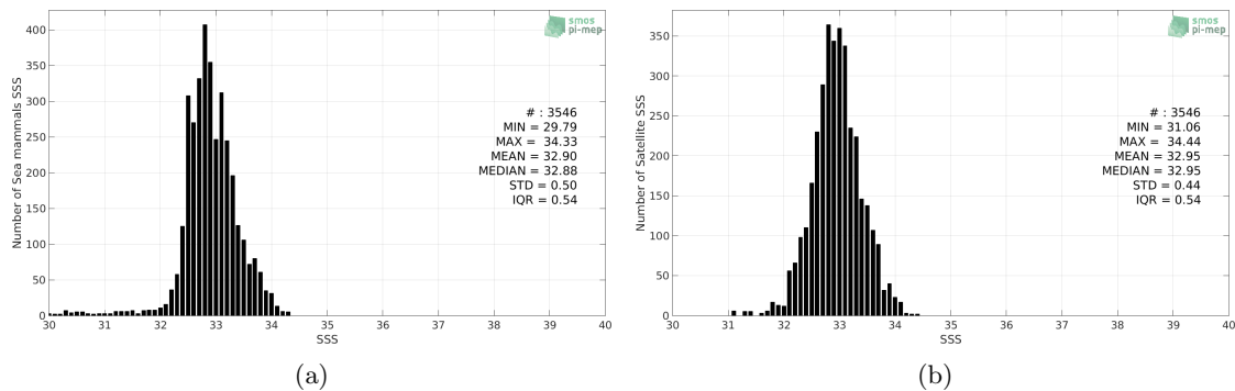
Figure 2: Histograms of SSS from Sea mammals (a) and Aquarius-L3-OR-V5-7DAY-RUNNING-1DEG (b) considering all match-up pairs per bins of 0.1 over the North Pacific Ocean Pi-MEP region and for the full satellite product period.
