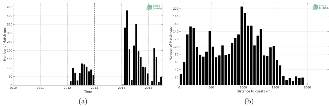
Figure 1: Number of match-ups between Sea mammals and Aquarius-L3-OR-V5-7DAY-RUNNING-1DEG SSS as a function of time (a) and as function of the distance to coast (b) over the North Pacific Ocean Pi-MEP region and for the full satellite product period.
