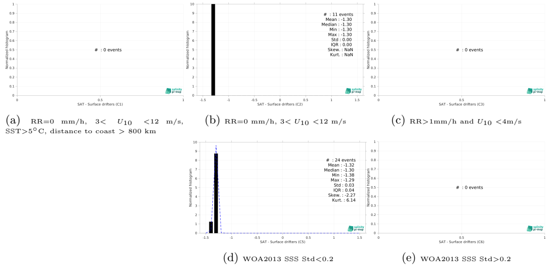
Figure 14: Normalized histogram of \Delta SSS (Aquarius SSS L3 OR v5 - 7-Day running (NASA-GSFC) - Surface drifters) for 5 different subdatasets corresponding to: RR=0 mm/h, 3 < U_{10} < 12 m/s, SST>5°C, distance to coast > 800 km (a), RR=0 mm/h, 3 < U_{10} < 12 m/s (b), RR>1mm/h and U_{10} < 4 m/s (c), WOA2013 SSS Std<0.2 (d), WOA2013 SSS Std>0.2 (e).
