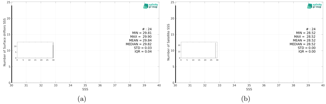
Figure 3: Histograms of SSS from Surface drifters (a) and Aquarius SSS L3 OR v5 - 7-Day running (NASA-GSFC) (b) considering all match-up pairs per bins of 0.1 over the North Pacific Ocean Pi-MEP region and for the full satellite product period.
