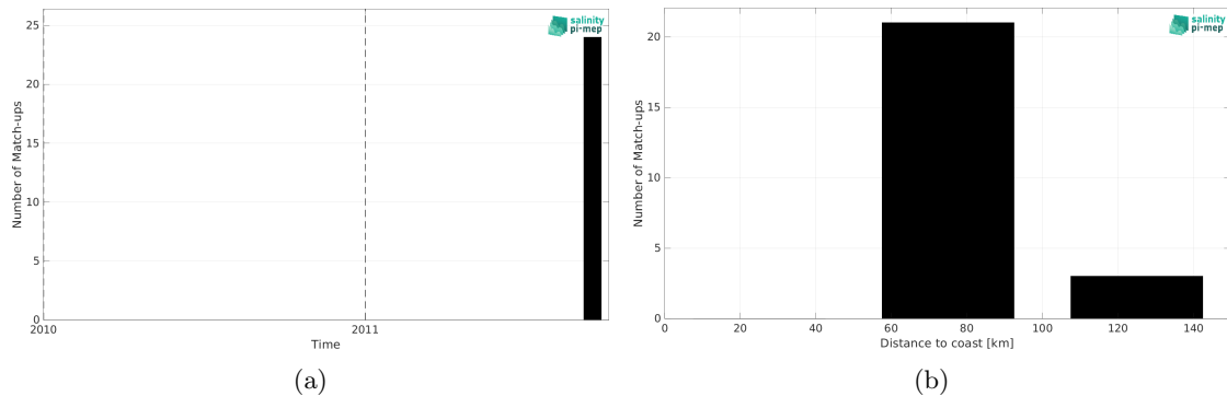
Figure 2: Number of match-ups between Surface drifters and Aquarius SSS L3 OR v5 - 7-Day running (NASA-GSFC) SSS as a function of time (a) and as function of the distance to coast (b) over the North Pacific Ocean Pi-MEP region and for the full satellite product period.
