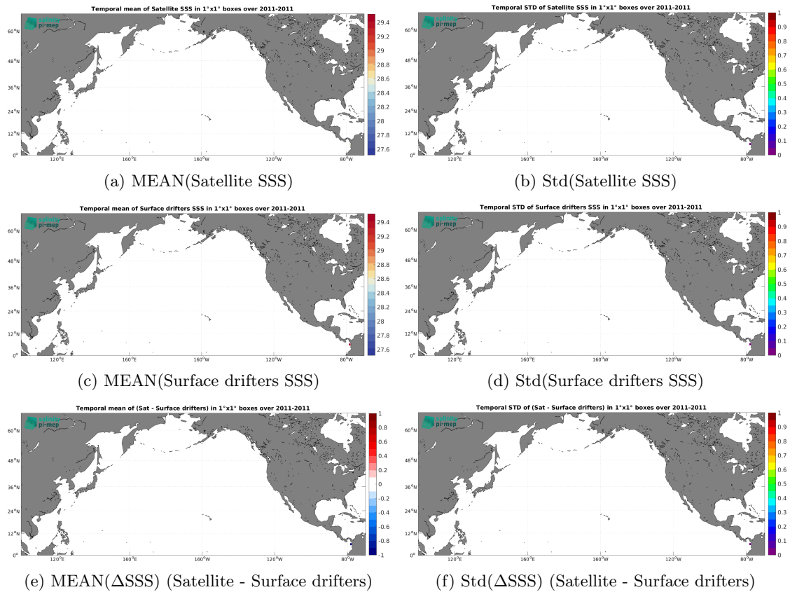
Figure 6: Temporal mean (left) and Std (right) of SSS from Aquarius SSS L3 OR v5 - 7-Day running (NASA-GSFC) (top), Surface drifters (middle), and of \Delta SSS (Satellite - Surface drifters). Only match-up pairs are used to generate these maps.
