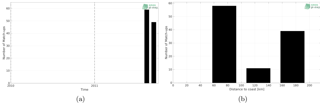
Figure 1: Number of match-ups between Surface drifters and Aquarius SSS L3 OR v5 - 7-Day running (NASA-GSFC) SSS as a function of time (a) and as function of the distance to coast (b) over the North Pacific Ocean Pi-MEP region and for the full satellite product period.
