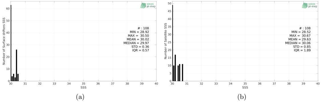
Figure 2: Histograms of SSS from Surface drifters (a) and Aquarius SSS L3 OR v5 - 7-Day running (NASA-GSFC) (b) considering all match-up pairs per bins of 0.1 over the North Pacific Ocean Pi-MEP region and for the full satellite product period.
