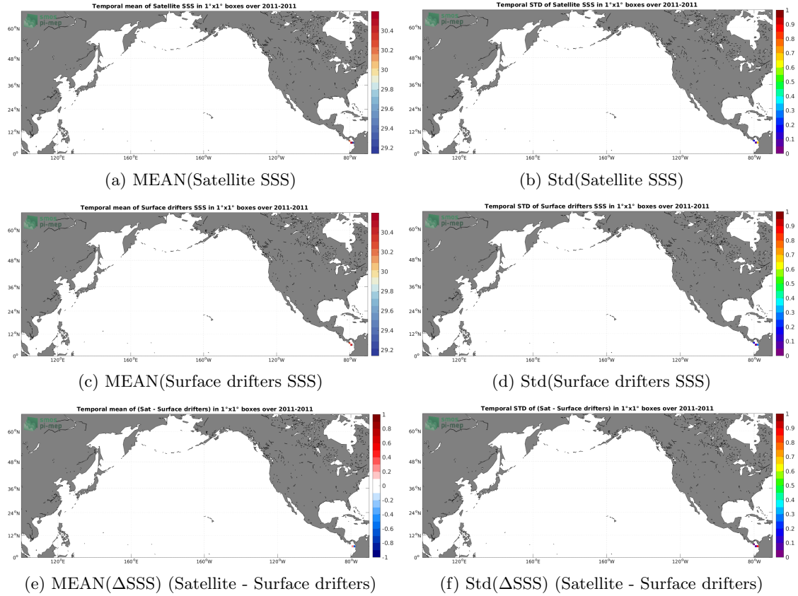
Figure 5: Temporal mean (left) and Std (right) of SSS from Aquarius SSS L3 OR v5 - 7-Day running (NASA-GSFC) (top), Surface drifters (middle), and of \Delta SSS (Satellite - Surface drifters). Only match-up pairs are used to generate these maps.
