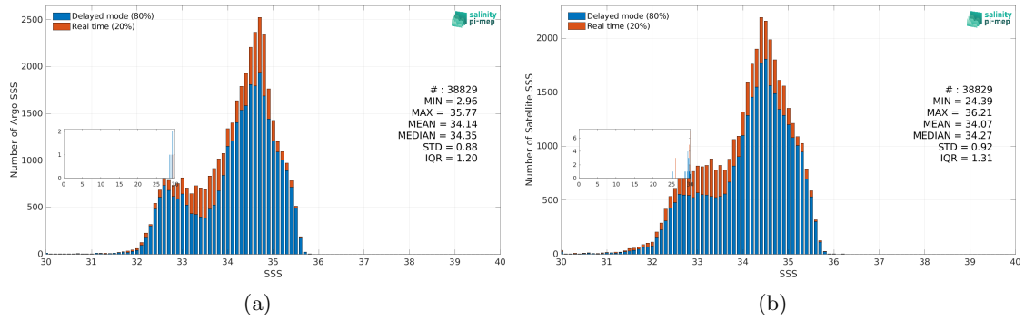
Figure 3: Histograms of SSS from Argo (a) and Aquarius SSS L3 OR v5 - 7-Day running (NASA-GSFC) (b) considering all match-up pairs per bins of 0.1 over the North Pacific Ocean Pi-MEP region and for the full satellite product period.
