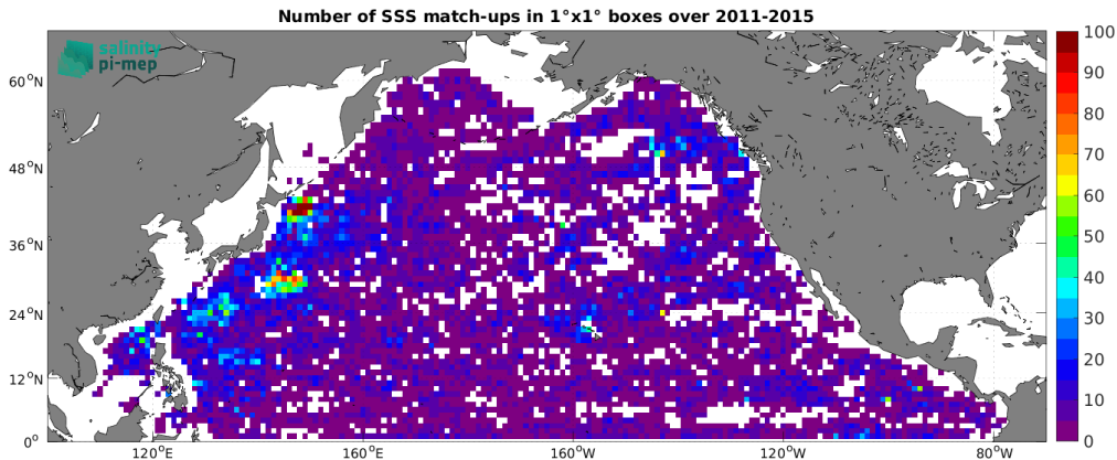
Figure 5: Number of SSS match-ups between Argo SSS and the Aquarius SSS L3 OR v5 - 7-Day running (NASA-GSFC) SSS product for the North Pacific Ocean Pi-MEP region over 1^\circ \times 1^\circ boxes and for the full satellite product period.
