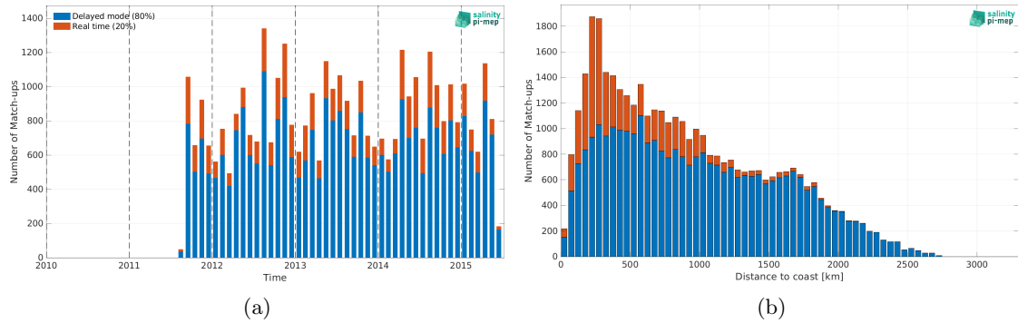
Figure 2: Number of match-ups between Argo and Aquarius SSS L3 OR v5 - 7-Day running (NASA-GSFC) SSS as a function of time (a) and as function of the distance to coast (b) over the North Pacific Ocean Pi-MEP region and for the full satellite product period.
