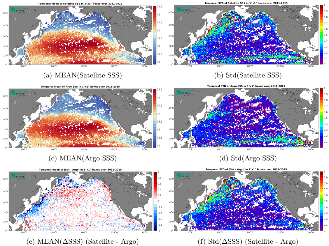
Figure 7: Temporal mean (left) and Std (right) of SSS from Aquarius SSS L3 OR v5 - 7-Day running (NASA-GSFC) (top), Argo (middle), and of \Delta SSS (Satellite - Argo). Only match-up pairs are used to generate these maps.
