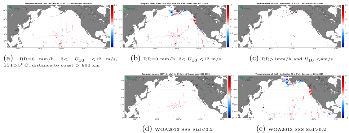
Figure 12: Temporal mean gridded over spatial boxes of size 1^\circ \times 1^\circ of \Delta SSS (Aquarius SSS L3 OR v5 - 7-Day running - Rain mask (NASA-GSFC) - TSG (SAMOS)) for 5 different subdatasets corresponding to:RR=0 mm/h, 3 < U_{10} < 12 m/s, SST >5^\circ C, distance to coast > 800 km (a), RR=0 mm/h, 3 < U_{10} < 12 m/s (b), RR >1 mm/h and U_{10} < 4 m/s (c), WOA2013 SSS Std <0.2 (d), WOA2013 SSS Std >0.2 (e).
