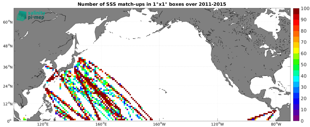
Figure 5: Number of SSS match-ups between TSG (LEGOS-DM) SSS and the Aquarius SSS L3 OR v5 - 7-Day running - Rain mask (NASA-GSFC) SSS product for the North Pacific Ocean Pi-MEP region over 1^\circ \times 1^\circ boxes and for the full satellite product period.
