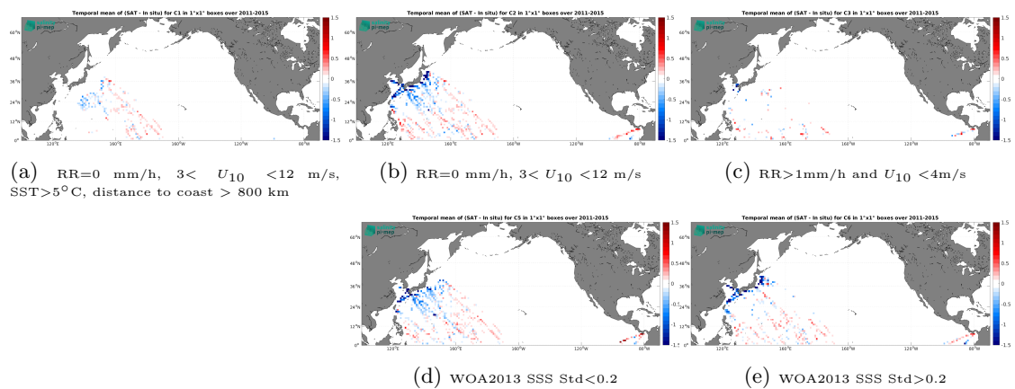
Figure 14: Temporal mean gridded over spatial boxes of size 1^\circ \times 1^\circ of \Delta\text{SSS} (Aquarius SSS L3 OR v5 - 7-Day running - Rain mask (NASA-GSFC) - TSG (LEGOS-DM)) for 5 different subdatasets corresponding to:RR=0 mm/h, 3 < U_{10} < 12 m/s, SST >5^\circ\text{C} , distance to coast > 800 km (a), RR=0 mm/h, 3 < U_{10} < 12 m/s (b), RR >1 mm/h and U_{10} < 4 m/s (c), WOA2013 SSS Std <0.2 (d), WOA2013 SSS Std >0.2 (e).
