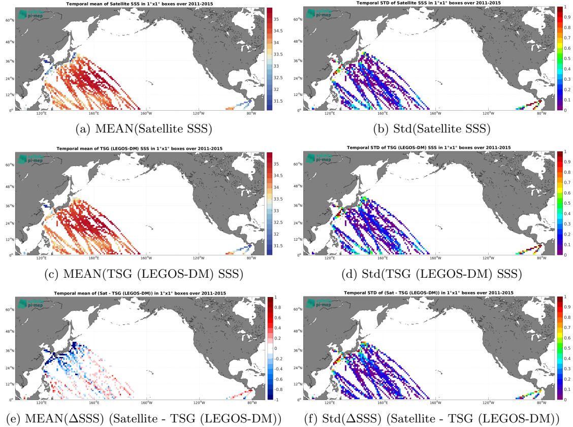
Figure 7: Temporal mean (left) and Std (right) of SSS from Aquarius SSS L3 OR v5 - 7-Day running - Rain mask (NASA-GSFC) (top), TSG (LEGOS-DM) (middle), and of \Delta SSS (Satellite - TSG (LEGOS-DM)). Only match-up pairs are used to generate these maps.
