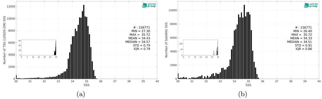
Figure 3: Histograms of SSS from TSG (LEGOS-DM) (a) and Aquarius SSS L3 OR v5 - 7-Day running - Rain mask (NASA-GSFC) (b) considering all match-up pairs per bins of 0.1 over the North Pacific Ocean Pi-MEP region and for the full satellite product period.
