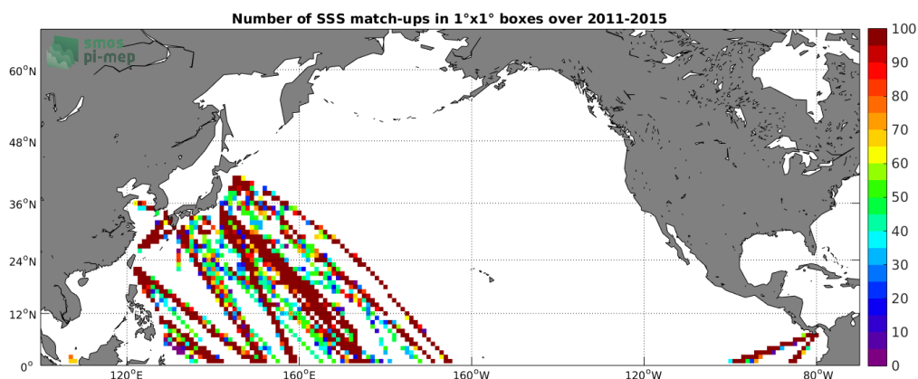
Figure 4: Number of SSS match-ups between TSG-LEGOS-DM SSS and the Aquarius-L3-OR-V5-7DAY-RUNNING-RAIN-MASK-1DEG SSS product for the North Pacific Ocean Pi-MEP region over 1^\circ \times 1^\circ boxes and for the full satellite product period.
