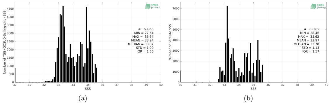
Figure 2: Histograms of SSS from TSG (GOSUD-Sailing-ship) (a) and Aquarius SSS L3 OR v5 - 7-Day running - Rain mask (NASA-GSFC) (b) considering all match-up pairs per bins of 0.1 over the North Pacific Ocean Pi-MEP region and for the full satellite product period.
