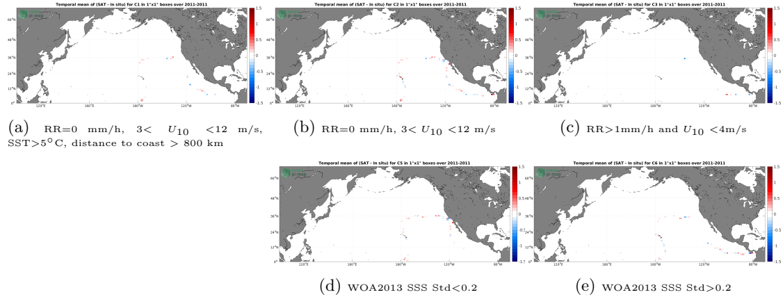
Figure 12: Temporal mean gridded over spatial boxes of size 1^{\circ}\times 1^{\circ} of \Delta SSS (Aquarius SSS L3 OR v5 - 7-Day running - Rain mask (NASA-GSFC) - TSG (GOSUD-Sailing-ship)) for 5 different subdatasets corresponding to:RR=0 mm/h, 3 < U_{10} < 12 m/s, SST >5^{\circ}\text{C} , distance to coast > 800 km (a), RR=0 mm/h, 3 < U_{10} < 12 m/s (b), RR >1 mm/h and U_{10} < 4 m/s (c), WOA2013 SSS Std <0.2 (d), WOA2013 SSS Std >0.2 (e).
