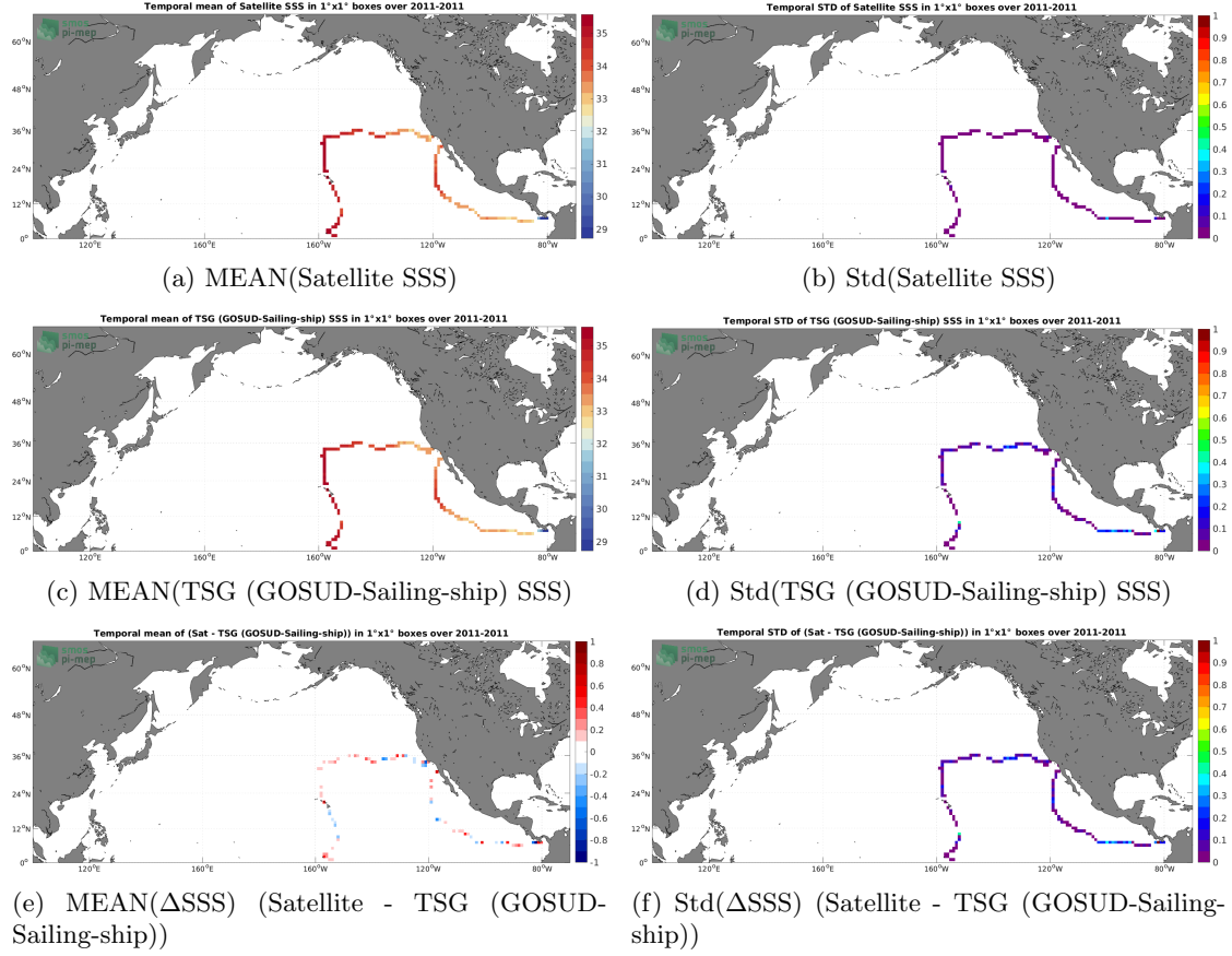
Figure 6: Temporal mean (left) and Std (right) of SSS from Aquarius SSS L3 OR v5 - 7-Day running - Rain mask (NASA-GSFC) (top), TSG (GOSUD-Sailing-ship) (middle), and of \Delta SSS (Satellite - TSG (GOSUD-Sailing-ship)). Only match-up pairs are used to generate these maps.
