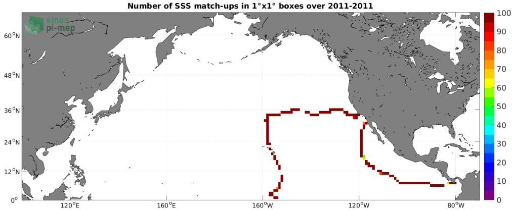
Figure 4: Number of SSS match-ups between TSG (GOSUD-Sailing-ship) SSS and the Aquarius SSS L3 OR v5 - 7-Day running - Rain mask (NASA-GSFC) SSS product for the North Pacific Ocean Pi-MEP region over 1^\circ \times 1^\circ boxes and for the full satellite product period.
