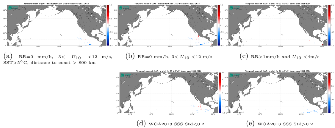
Figure 14: Temporal mean gridded over spatial boxes of size 1^\circ \times 1^\circ of \Delta\text{SSS} (Aquarius SSS L3 OR v5 - 7-Day running - Rain mask (NASA-GSFC) - TSG (GOSUD-Research-vessel)) for 5 different subdatasets corresponding to: RR=0 mm/h, 3 < U_{10} < 12 m/s, SST > 5°C, distance to coast > 800 km (a), RR=0 mm/h, 3 < U_{10} < 12 m/s (b), RR > 1mm/h and U_{10} < 4 m/s (c), WOA2013 SSS Std < 0.2 (d), WOA2013 SSS Std > 0.2 (e).
