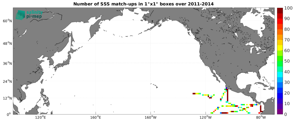
Figure 5: Number of SSS match-ups between TSG (GOSUD-Research-vessel) SSS and the Aquarius SSS L3 OR v5 - 7-Day running - Rain mask (NASA-GSFC) SSS product for the North Pacific Ocean Pi-MEP region over 1^\circ \times 1^\circ boxes and for the full satellite product period.
