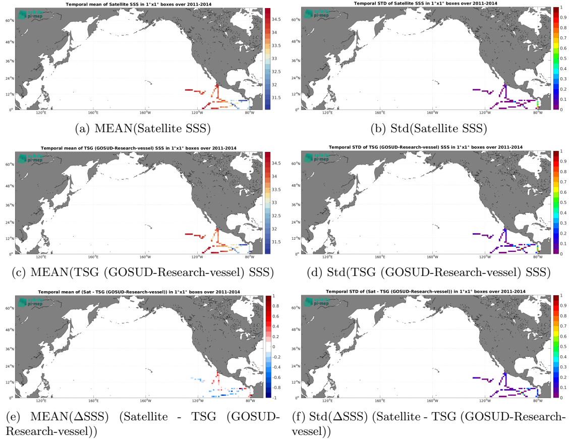
Figure 7: Temporal mean (left) and Std (right) of SSS from Aquarius SSS L3 OR v5 - 7-Day running - Rain mask (NASA-GSFC) (top), TSG (GOSUD-Research-vessel) (middle), and of \Delta SSS (Satellite - TSG (GOSUD-Research-vessel)). Only match-up pairs are used to generate these maps.
