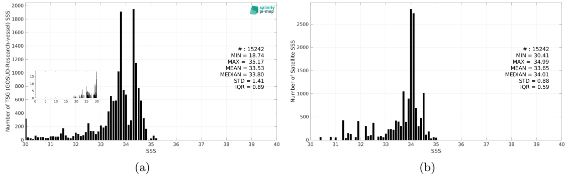
Figure 3: Histograms of SSS from TSG (GOSUD-Research-vessel) (a) and Aquarius SSS L3 OR v5 - 7-Day running - Rain mask (NASA-GSFC) (b) considering all match-up pairs per bins of 0.1 over the North Pacific Ocean Pi-MEP region and for the full satellite product period.
