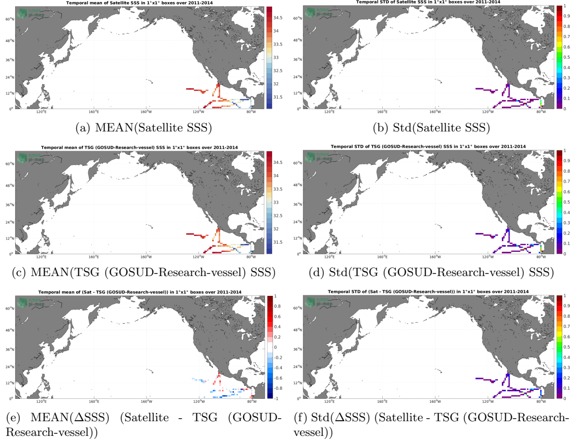
Figure 6: Temporal mean (left) and Std (right) of SSS from Aquarius SSS L3 OR v5 - 7-Day running - Rain mask (NASA-GSFC) (top), TSG (GOSUD-Research-vessel) (middle), and of \Delta SSS (Satellite - TSG (GOSUD-Research-vessel)). Only match-up pairs are used to generate these maps.
