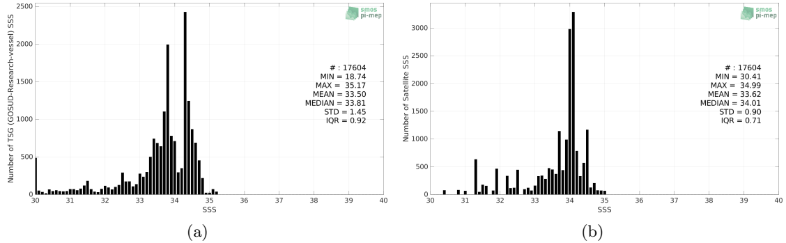
Figure 2: Histograms of SSS from TSG (GOSUD-Research-vessel) (a) and Aquarius SSS L3 OR v5 - 7-Day running - Rain mask (NASA-GSFC) (b) considering all match-up pairs per bins of 0.1 over the North Pacific Ocean Pi-MEP region and for the full satellite product period.
