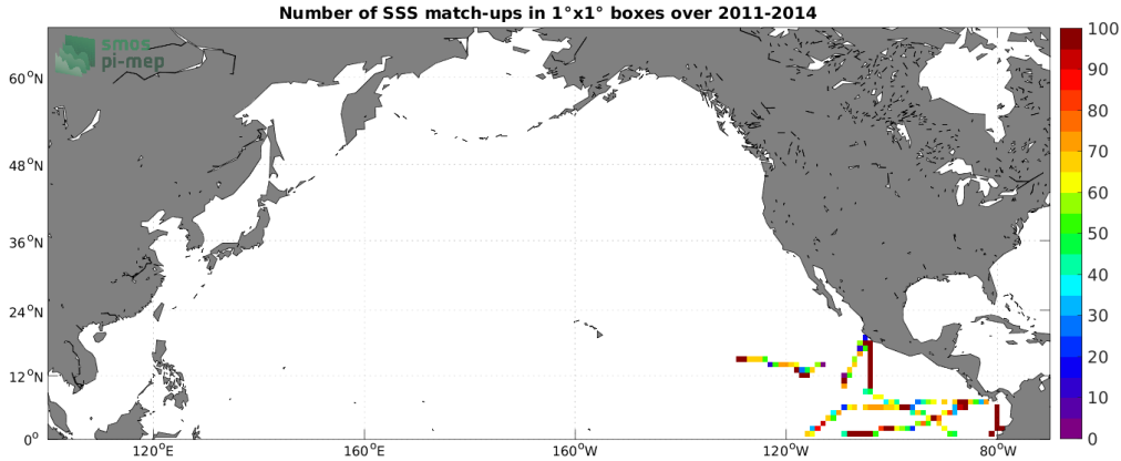
Figure 4: Number of SSS match-ups between TSG (GOSUD-Research-vessel) SSS and the Aquarius SSS L3 OR v5 - 7-Day running - Rain mask (NASA-GSFC) SSS product for the North Pacific Ocean Pi-MEP region over 1^\circ \times 1^\circ boxes and for the full satellite product period.
