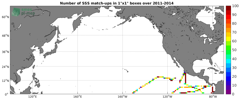
Figure 4: Number of SSS match-ups between TSG-GOSUD-Research-vessel SSS and the Aquarius-L3-OR-V5-7DAY-RUNNING-RAIN-MASK-1DEG SSS product for the North Pacific Ocean Pi-MEP region over 1^\circ \times 1^\circ boxes and for the full satellite product period.
