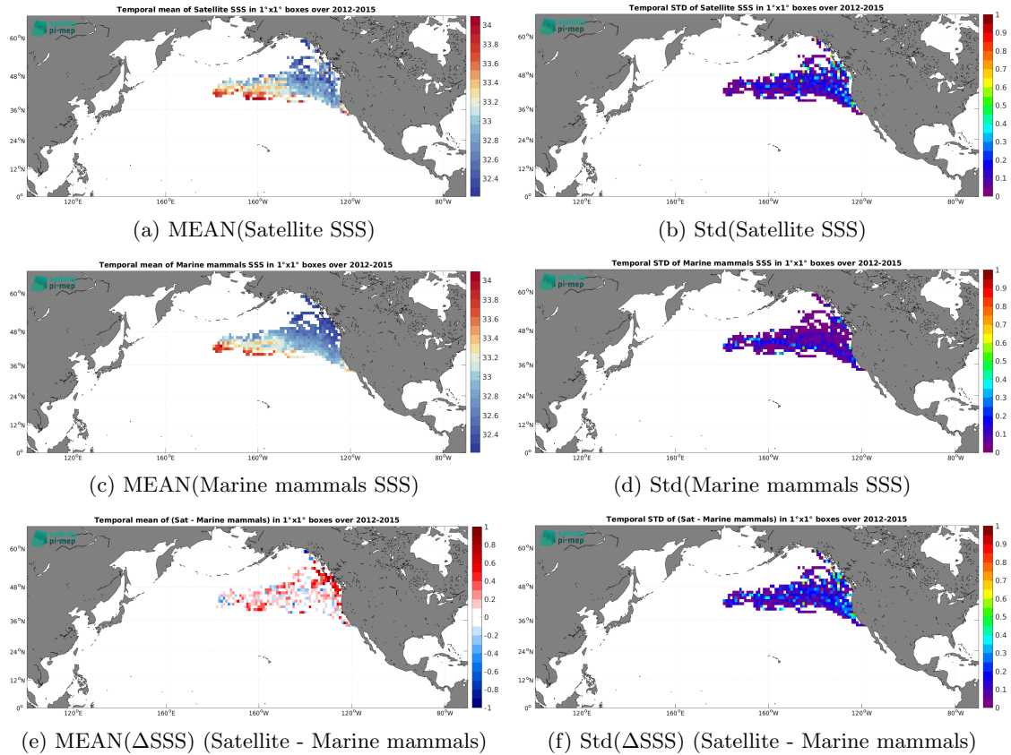
Figure 7: Temporal mean (left) and Std (right) of SSS from Aquarius SSS L3 OR v5 - 7-Day running - Rain mask (NASA-GSFC) (top), Marine mammals (middle), and of \Delta SSS (Satellite - Marine mammals). Only match-up pairs are used to generate these maps.
