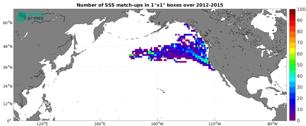
Figure 5: Number of SSS match-ups between Marine mammals SSS and the Aquarius SSS L3 OR v5 - 7-Day running - Rain mask (NASA-GSFC) SSS product for the North Pacific Ocean Pi-MEP region over 1^\circ \times 1^\circ boxes and for the full satellite product period.
