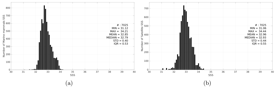
Figure 3: Histograms of SSS from Marine mammals (a) and Aquarius SSS L3 OR v5 - 7-Day running - Rain mask (NASA-GSFC) (b) considering all match-up pairs per bins of 0.1 over the North Pacific Ocean Pi-MEP region and for the full satellite product period.
