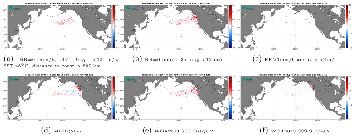
Figure 14: Temporal mean gridded over spatial boxes of size 1^\circ \times 1^\circ of \Delta SSS (Aquarius SSS L3 OR v5 - 7-Day running - Rain mask (NASA-GSFC) - Marine mammals) for 6 different subdatasets corresponding to:RR=0 mm/h, 3 < U_{10} < 12 m/s, SST >5^\circ C, distance to coast > 800 km (a), RR=0 mm/h, 3 < U_{10} < 12 m/s (b), RR >1 mm/h and U_{10} < 4 m/s (c),MLD <20 m (d),WOA2013 SSS Std <0.2 (e),WOA2013 SSS Std >0.2 (f).
