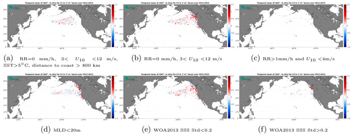
Figure 12: Temporal mean gridded over spatial boxes of size 1^{\circ}\times 1^{\circ} of \Delta\text{SSS} (Aquarius SSS L3 OR v5 - 7-Day running - Rain mask (NASA-GSFC) - Marine mammals) for 6 different subdatasets corresponding to: RR=0 mm/h, 3 < U_{10} < 12 m/s, SST > 5^{\circ}\text{C} , distance to coast > 800 km (a), RR=0 mm/h, 3 < U_{10} < 12 m/s (b), RR > 1 mm/h and U_{10} < 4 m/s (c), MLD < 20\text{m} (d), WOA2013 SSS Std < 0.2 (e), WOA2013 SSS Std > 0.2 (f).
