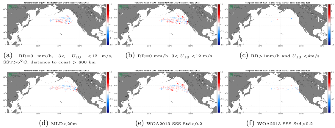
Figure 12: Temporal mean gridded over spatial boxes of size 1^{\circ} \times 1^{\circ} of \Delta\text{SSS} (Aquarius SSS L3 OR v5 - 7-Day running - Rain mask (NASA-GSFC) - Marine mammals) for 6 different subdatasets corresponding to: RR=0 mm/h, 3 < U_{10} < 12 m/s, SST > 5^{\circ}\text{C} , distance to coast > 800 km (a), RR=0 mm/h, 3 < U_{10} < 12 m/s (b), RR > 1 mm/h and U_{10} < 4 m/s (c),MLD < 20\text{m} (d),WOA2013 SSS Std < 0.2 (e),WOA2013 SSS Std > 0.2 (f).
