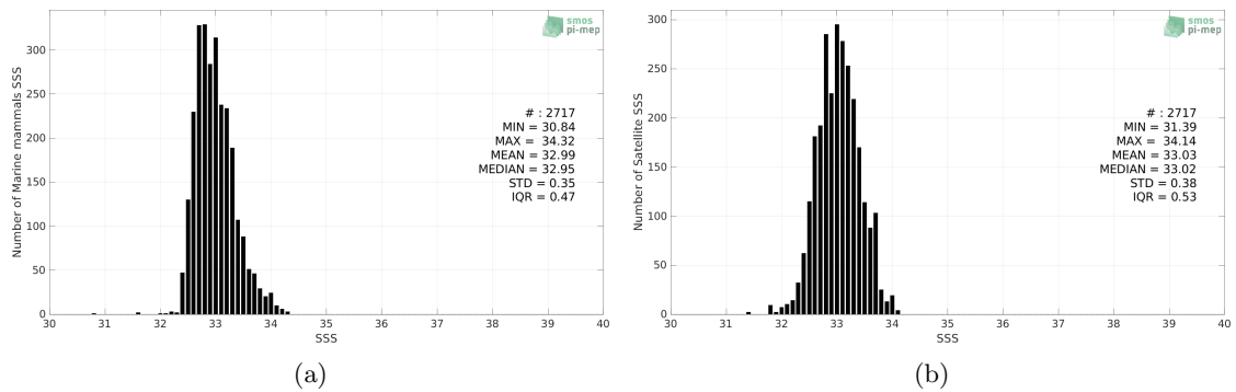
Figure 2: Histograms of SSS from Marine mammals (a) and Aquarius SSS L3 OR v5 - 7-Day running - Rain mask (NASA-GSFC) (b) considering all match-up pairs per bins of 0.1 over the North Pacific Ocean Pi-MEP region and for the full satellite product period.
