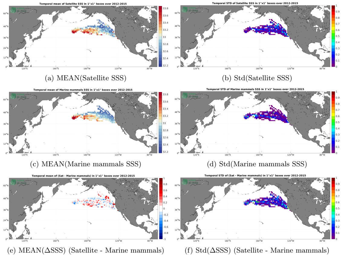
Figure 6: Temporal mean (left) and Std (right) of SSS from Aquarius SSS L3 OR v5 - 7-Day running - Rain mask (NASA-GSFC) (top), Marine mammals (middle), and of \Delta SSS (Satellite - Marine mammals). Only match-up pairs are used to generate these maps.
