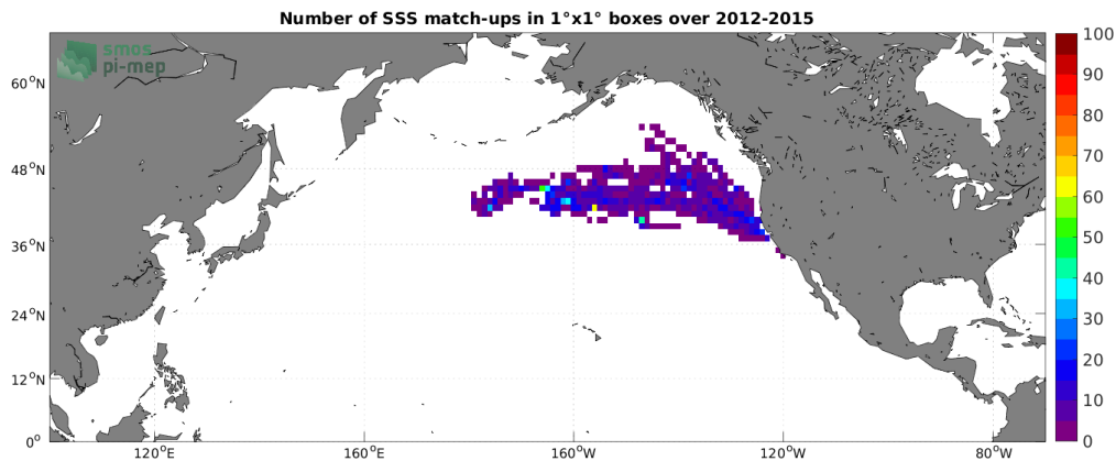
Figure 4: Number of SSS match-ups between Marine mammals SSS and the Aquarius SSS L3 OR v5 - 7-Day running - Rain mask (NASA-GSFC) SSS product for the North Pacific Ocean Pi-MEP region over 1^\circ \times 1^\circ boxes and for the full satellite product period.
