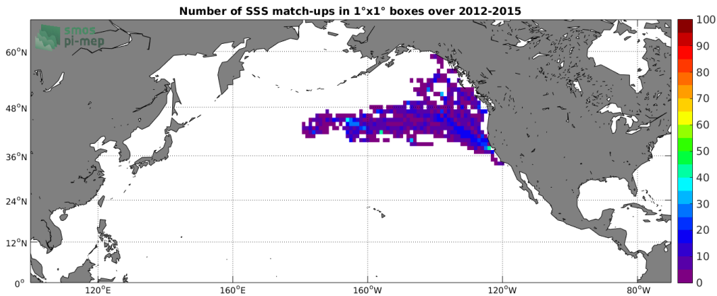
Figure 4: Number of SSS match-ups between Sea mammals SSS and the Aquarius-L3-OR-V5-7DAY-RUNNING-RAIN-MASK-1DEG SSS product for the North Pacific Ocean Pi-MEP region over 1°x1° boxes and for the full satellite product period.
