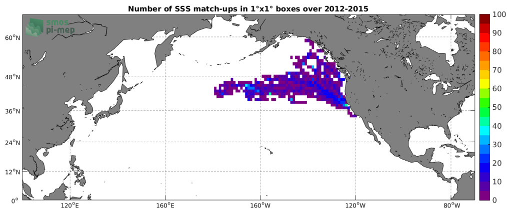
Figure 4: Number of SSS match-ups between Sea mammals SSS and the Aquarius-L3-OR-V5-7DAY-RUNNING-RAIN-MASK-1DEG SSS product for the North Pacific Ocean Pi-MEP region over 1^\circ \times 1^\circ boxes and for the full satellite product period.
