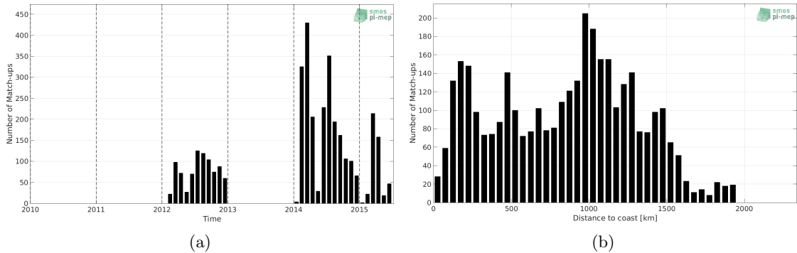
Figure 1: Number of match-ups between Sea mammals and Aquarius-L3-OR-V5-7DAY-RUNNING-RAIN-MASK-1DEG SSS as a function of time (a) and as function of the distance to coast (b) over the North Pacific Ocean Pi-MEP region and for the full satellite product period.
