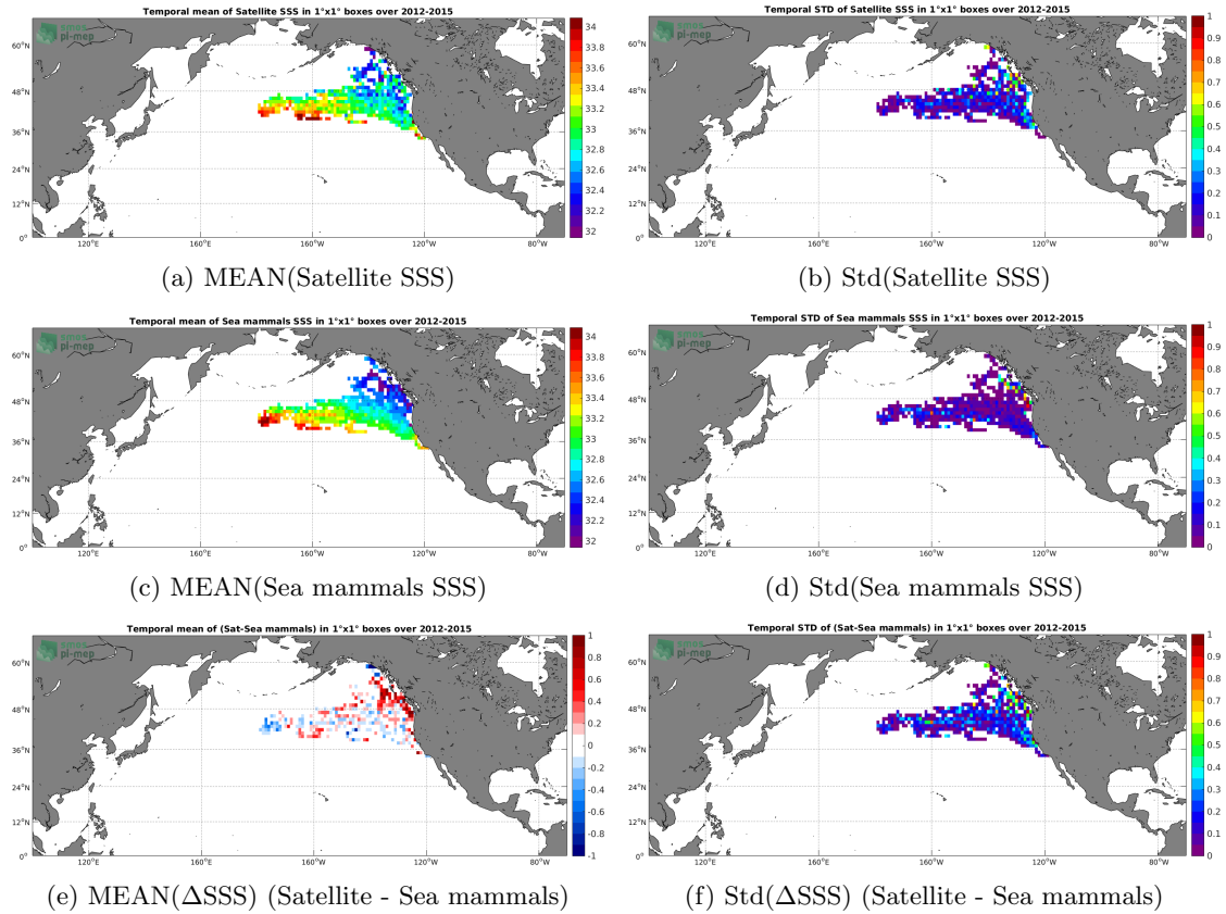
Figure 6: Temporal mean (left) and Std (right) of SSS from Aquarius-L3-OR-V5-7DAY-RUNNING-RAIN-MASK-1DEG (top), Sea mammals (middle), and of \Delta SSS (Satellite - Sea mammals). Only match-up pairs are used to generate these maps.
