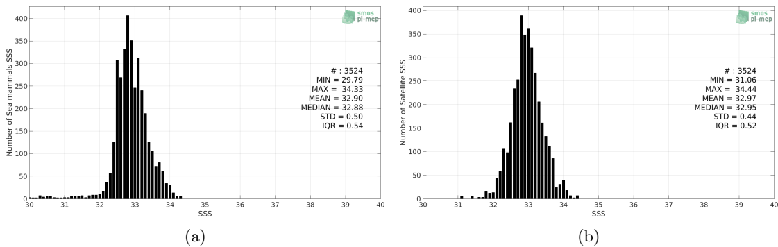
Figure 2: Histograms of SSS from Sea mammals (a) and Aquarius-L3-OR-V5-7DAY-RUNNING-RAIN-MASK-1DEG (b) considering all match-up pairs per bins of 0.1 over the North Pacific Ocean Pi-MEP region and for the full satellite product period.
