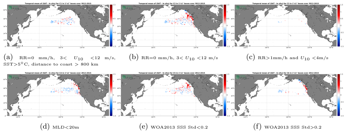
Figure 12: Temporal mean gridded over spatial boxes of size 1^\circ \times 1^\circ of \Delta SSS (Aquarius-L3-OR-V5-7DAY-RUNNING-RAIN-MASK-1DEG - Sea mammals) for 6 different subdatasets corresponding to:RR=0 mm/h, 3 < U_{10} < 12 m/s, SST >5^\circ C, distance to coast > 800 km (a), RR=0 mm/h, 3 < U_{10} < 12 m/s (b), RR >1 mm/h and U_{10} < 4 m/s (c),MLD <20 m (d),WOA2013 SSS Std <0.2 (e),WOA2013 SSS Std >0.2 (f).
