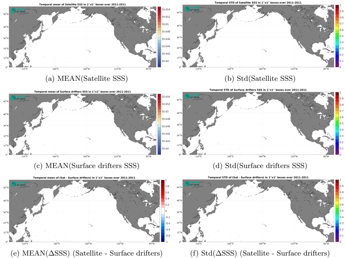
Figure 6: Temporal mean (left) and Std (right) of SSS from Aquarius SSS L3 OR v5 - 7-Day running - Rain mask (NASA-GSFC) (top), Surface drifters (middle), and of \Delta SSS (Satellite - Surface drifters). Only match-up pairs are used to generate these maps.
