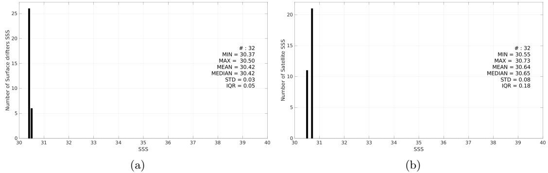
Figure 3: Histograms of SSS from Surface drifters (a) and Aquarius SSS L3 OR v5 - 7-Day running - Rain mask (NASA-GSFC) (b) considering all match-up pairs per bins of 0.1 over the North Pacific Ocean Pi-MEP region and for the full satellite product period.
