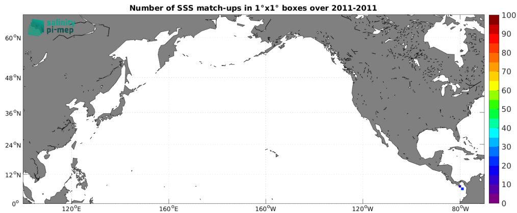
Figure 4: Number of SSS match-ups between Surface drifters SSS and the Aquarius SSS L3 OR v5 - 7-Day running - Rain mask (NASA-GSFC) SSS product for the North Pacific Ocean Pi-MEP region over 1^\circ \times 1^\circ boxes and for the full satellite product period.
