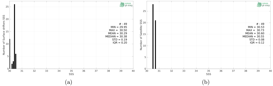
Figure 2: Histograms of SSS from Surface drifters (a) and Aquarius SSS L3 OR v5 - 7-Day running - Rain mask (NASA-GSFC) (b) considering all match-up pairs per bins of 0.1 over the North Pacific Ocean Pi-MEP region and for the full satellite product period.
