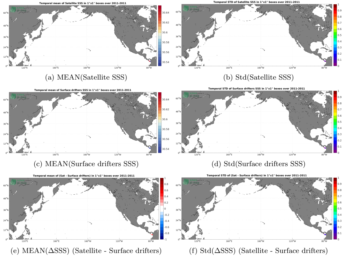
Figure 5: Temporal mean (left) and Std (right) of SSS from Aquarius SSS L3 OR v5 - 7-Day running - Rain mask (NASA-GSFC) (top), Surface drifters (middle), and of \Delta SSS (Satellite - Surface drifters). Only match-up pairs are used to generate these maps.
