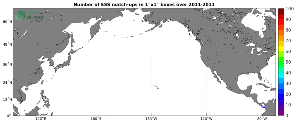
Figure 3: Number of SSS match-ups between Surface drifters SSS and the Aquarius SSS L3 OR v5 - 7-Day running - Rain mask (NASA-GSFC) SSS product for the North Pacific Ocean Pi-MEP region over 1^\circ \times 1^\circ boxes and for the full satellite product period.
