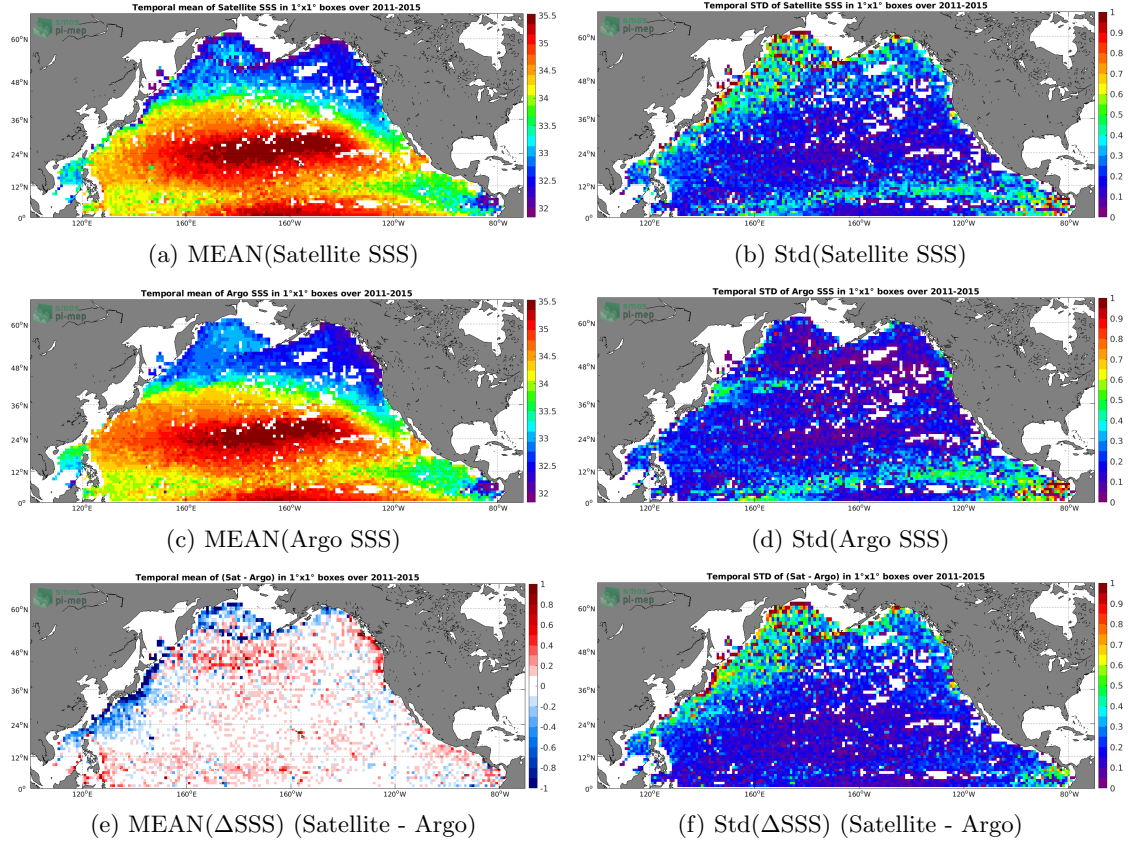
Figure 6: Temporal mean (left) and Std (right) of SSS from Aquarius SSS L3 OR v5 - 7-Day running - Rain mask (NASA-GSFC) (top), Argo (middle), and of \Delta\text{SSS} (Satellite - Argo). Only match-up pairs are used to generate these maps.
