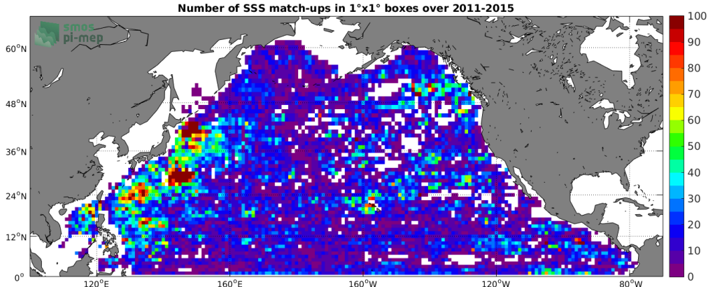
Figure 4: Number of SSS match-ups between Argo SSS and the Aquarius-L3-OR-V5-7DAY-RUNNING-RAIN-MASK-1DEG SSS product for the North Pacific Ocean Pi-MEP region over 1^\circ \times 1^\circ boxes and for the full satellite product period.
