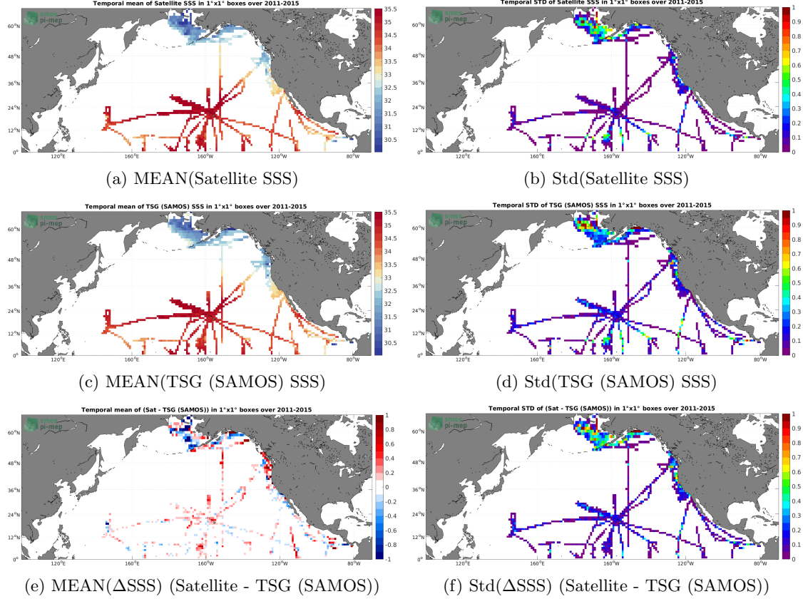
Figure 6: Temporal mean (left) and Std (right) of SSS from Aquarius SSS L3 OR v5 - Monthly (NASA-GSFC) (top), TSG (SAMOS) (middle), and of \Delta\text{SSS} (Satellite - TSG (SAMOS)). Only match-up pairs are used to generate these maps.
