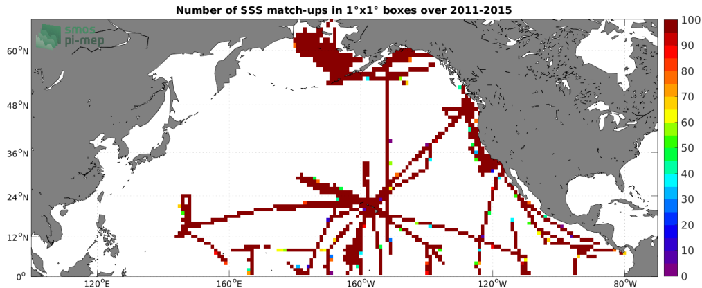
Figure 4: Number of SSS match-ups between TSG (SAMOS) SSS and the Aquarius SSS L3 OR v5 - Monthly (NASA-GSFC) SSS product for the North Pacific Ocean Pi-MEP region over 1^\circ \times 1^\circ boxes and for the full satellite product period.
