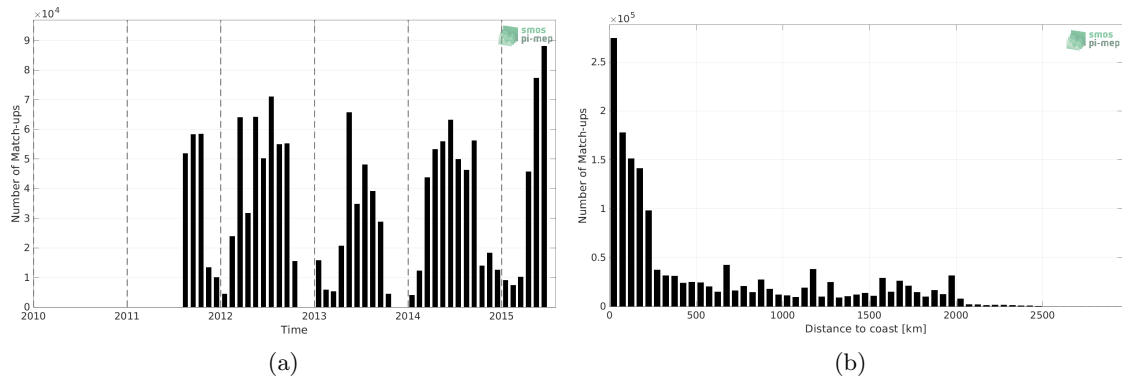
Figure 1: Number of match-ups between TSG (SAMOS) and Aquarius SSS L3 OR v5 - Monthly (NASA-GSFC) SSS as a function of time (a) and as function of the distance to coast (b) over the North Pacific Ocean Pi-MEP region and for the full satellite product period.
