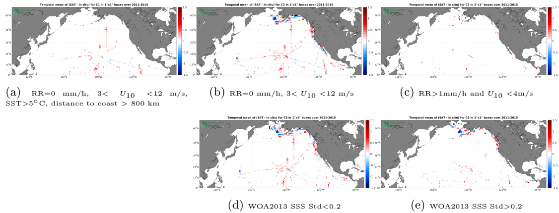
Figure 12: Temporal mean gridded over spatial boxes of size 1^\circ \times 1^\circ of \Delta SSS (Aquarius SSS L3 OR v5 - Monthly (NASA-GSFC) - TSG (SAMOS)) for 5 different subdatasets corresponding to:RR=0 mm/h, 3 < U_{10} < 12 m/s, SST >5^\circ C, distance to coast > 800 km (a), RR=0 mm/h, 3 < U_{10} < 12 m/s (b), RR >1 mm/h and U_{10} < 4 m/s (c), WOA2013 SSS Std <0.2 (d), WOA2013 SSS Std >0.2 (e).
