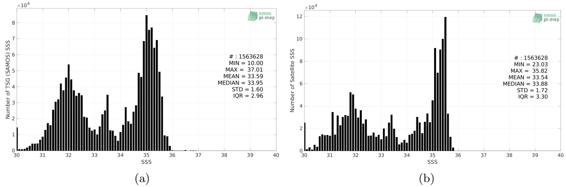
Figure 2: Histograms of SSS from TSG (SAMOS) (a) and Aquarius SSS L3 OR v5 - Monthly (NASA-GSFC) (b) considering all match-up pairs per bins of 0.1 over the North Pacific Ocean Pi-MEP region and for the full satellite product period.
