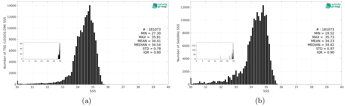
Figure 3: Histograms of SSS from TSG (LEGOS-DM) (a) and Aquarius SSS L3 OR v5 - Monthly (NASA-GSFC) (b) considering all match-up pairs per bins of 0.1 over the North Pacific Ocean Pi-MEP region and for the full satellite product period.
