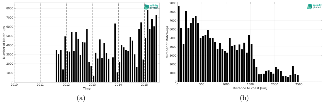
Figure 2: Number of match-ups between TSG (LEGOS-DM) and Aquarius SSS L3 OR v5 - Monthly (NASA-GSFC) SSS as a function of time (a) and as function of the distance to coast (b) over the North Pacific Ocean Pi-MEP region and for the full satellite product period.
