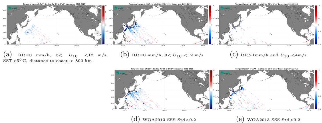
Figure 14: Temporal mean gridded over spatial boxes of size 1^\circ \times 1^\circ of \Delta\text{SSS} (Aquarius SSS L3 OR v5 - Monthly (NASA-GSFC) - TSG (LEGOS-DM)) for 5 different subdatasets corresponding to: RR=0 mm/h, 3 < U_{10} < 12 m/s, SST > 5°C, distance to coast > 800 km (a), RR=0 mm/h, 3 < U_{10} < 12 m/s (b), RR > 1 mm/h and U_{10} < 4 m/s (c), WOA2013 SSS Std < 0.2 (d), WOA2013 SSS Std > 0.2 (e).
