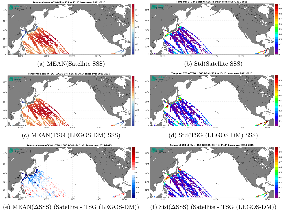
Figure 7: Temporal mean (left) and Std (right) of SSS from Aquarius SSS L3 OR v5 - Monthly (NASA-GSFC) (top), TSG (LEGOS-DM) (middle), and of \Delta\text{SSS} (Satellite - TSG (LEGOS-DM)). Only match-up pairs are used to generate these maps.
