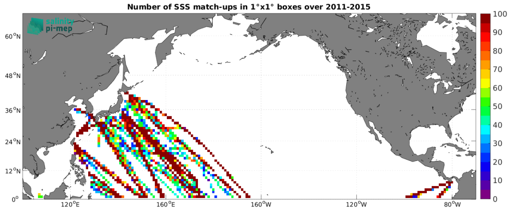
Figure 5: Number of SSS match-ups between TSG (LEGOS-DM) SSS and the Aquarius SSS L3 OR v5 - Monthly (NASA-GSFC) SSS product for the North Pacific Ocean Pi-MEP region over 1^\circ \times 1^\circ boxes and for the full satellite product period.
