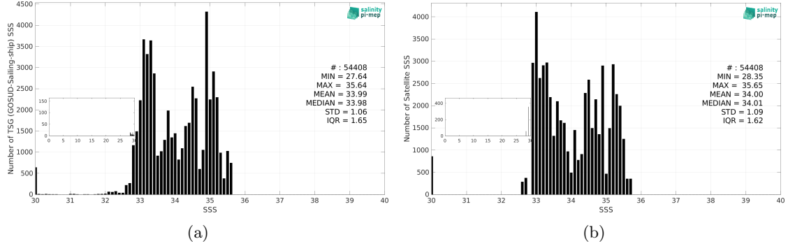
Figure 3: Histograms of SSS from TSG (GOSUD-Sailing-ship) (a) and Aquarius SSS L3 OR v5 - Monthly (NASA-GSFC) (b) considering all match-up pairs per bins of 0.1 over the North Pacific Ocean Pi-MEP region and for the full satellite product period.
