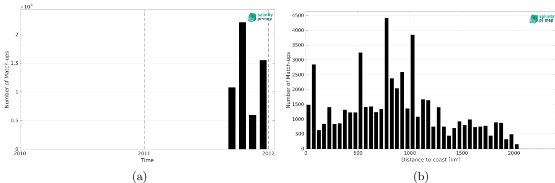
Figure 2: Number of match-ups between TSG (GOSUD-Sailing-ship) and Aquarius SSS L3 OR v5 - Monthly (NASA-GSFC) SSS as a function of time (a) and as function of the distance to coast (b) over the North Pacific Ocean Pi-MEP region and for the full satellite product period.
