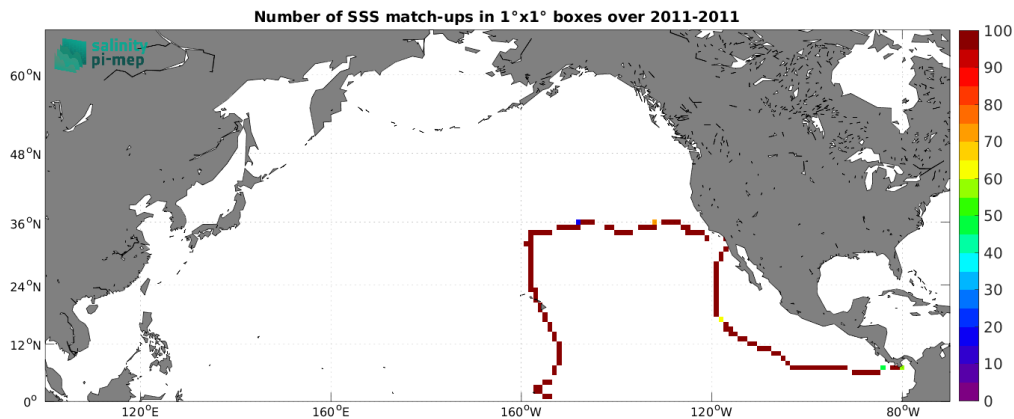
Figure 5: Number of SSS match-ups between TSG (GOSUD-Sailing-ship) SSS and the Aquarius SSS L3 OR v5 - Monthly (NASA-GSFC) SSS product for the North Pacific Ocean Pi-MEP region over 1^\circ \times 1^\circ boxes and for the full satellite product period.
