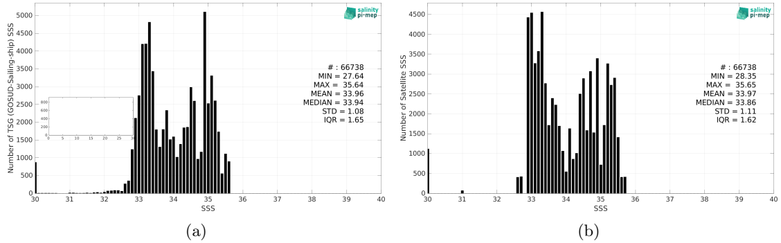
Figure 2: Histograms of SSS from TSG (GOSUD-Sailing-ship) (a) and Aquarius SSS L3 OR v5 - Monthly (NASA-GSFC) (b) considering all match-up pairs per bins of 0.1 over the North Pacific Ocean Pi-MEP region and for the full satellite product period.
