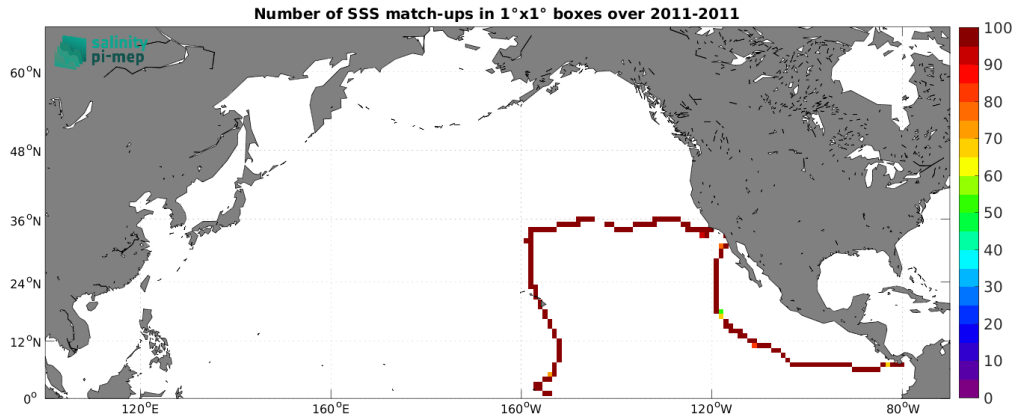
Figure 4: Number of SSS match-ups between TSG (GOSUD-Sailing-ship) SSS and the Aquarius SSS L3 OR v5 - Monthly (NASA-GSFC) SSS product for the North Pacific Ocean Pi-MEP region over 1^\circ \times 1^\circ boxes and for the full satellite product period.
