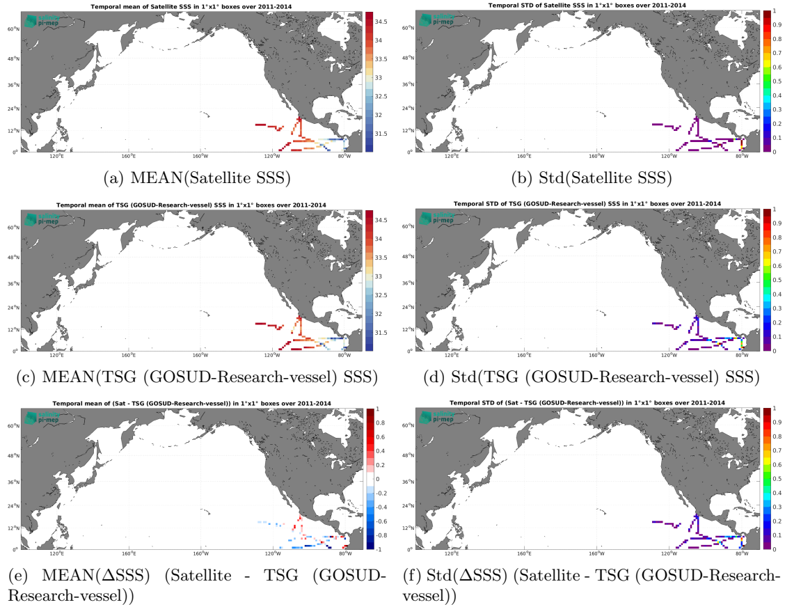
Figure 7: Temporal mean (left) and Std (right) of SSS from Aquarius SSS L3 OR v5 - Monthly (NASA-GSFC) (top), TSG (GOSUD-Research-vessel) (middle), and of \Delta SSS (Satellite - TSG (GOSUD-Research-vessel)). Only match-up pairs are used to generate these maps.
