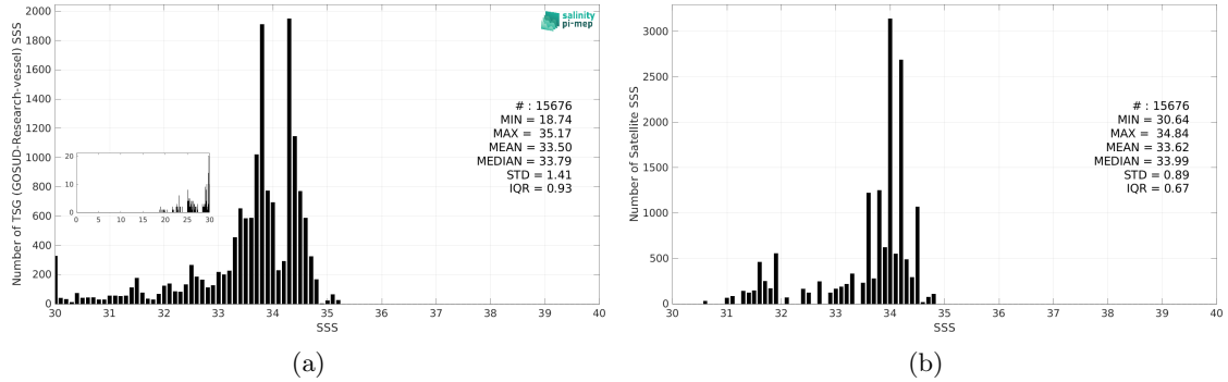
Figure 3: Histograms of SSS from TSG (GOSUD-Research-vessel) (a) and Aquarius SSS L3 OR v5 - Monthly (NASA-GSFC) (b) considering all match-up pairs per bins of 0.1 over the North Pacific Ocean Pi-MEP region and for the full satellite product period.
