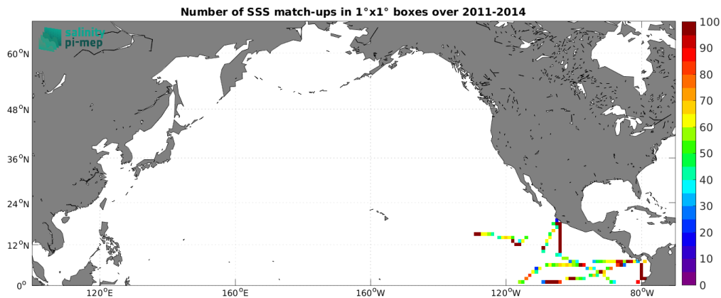
Figure 5: Number of SSS match-ups between TSG (GOSUD-Research-vessel) SSS and the Aquarius SSS L3 OR v5 - Monthly (NASA-GSFC) SSS product for the North Pacific Ocean Pi-MEP region over 1^\circ \times 1^\circ boxes and for the full satellite product period.
