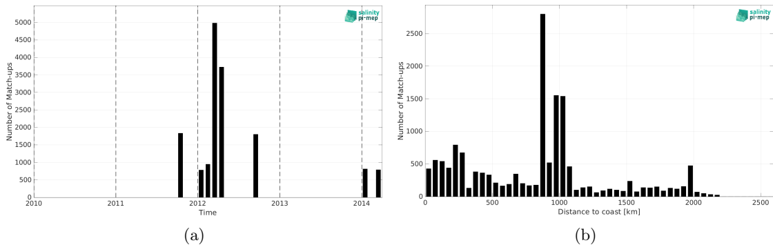
Figure 2: Number of match-ups between TSG (GOSUD-Research-vessel) and Aquarius SSS L3 OR v5 - Monthly (NASA-GSFC) SSS as a function of time (a) and as function of the distance to coast (b) over the North Pacific Ocean Pi-MEP region and for the full satellite product period.
