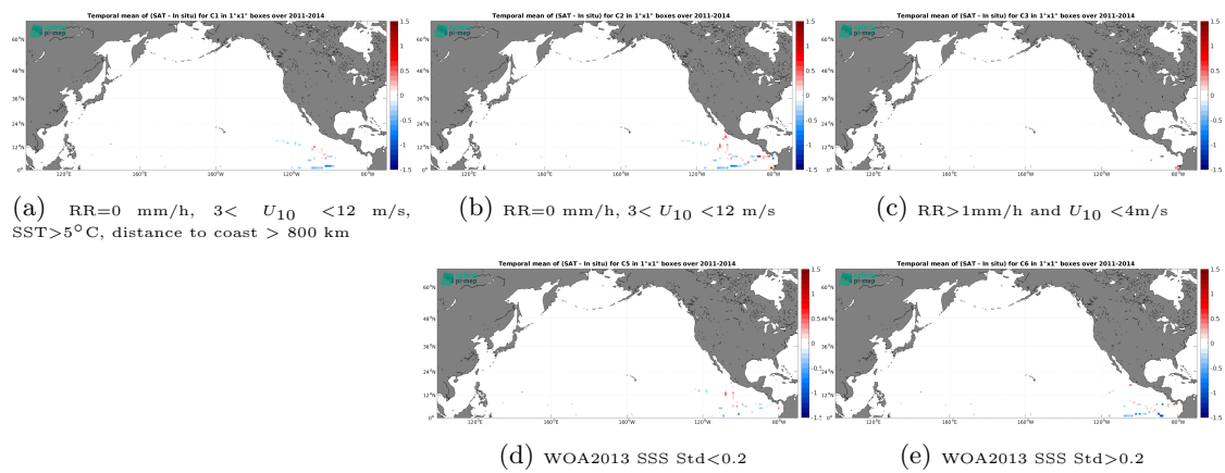
Figure 14: Temporal mean gridded over spatial boxes of size 1^\circ \times 1^\circ of \Delta SSS (Aquarius SSS L3 OR v5 - Monthly (NASA-GSFC) - TSG (GOSUD-Research-vessel)) for 5 different subdatasets corresponding to:RR=0 mm/h, 3 < U_{10} < 12 m/s, SST >5^\circ C, distance to coast > 800 km (a), RR=0 mm/h, 3 < U_{10} < 12 m/s (b), RR >1 mm/h and U_{10} < 4 m/s (c), WOA2013 SSS Std <0.2 (d), WOA2013 SSS Std >0.2 (e).
