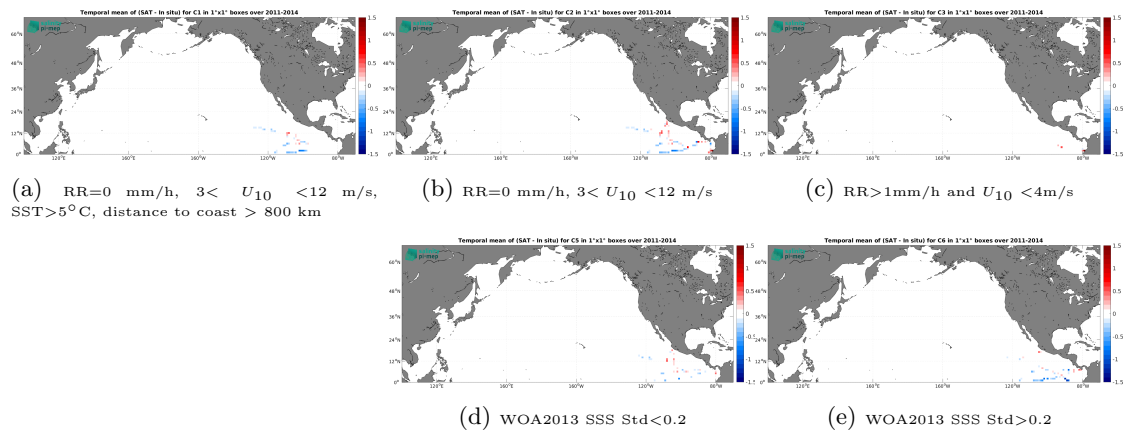
Figure 12: Temporal mean gridded over spatial boxes of size 1^\circ \times 1^\circ of \Delta\text{SSS} (Aquarius SSS L3 OR v5 - Monthly (NASA-GSFC) - TSG (GOSUD-Research-vessel)) for 5 different subdatasets corresponding to: RR=0 mm/h, 3 < U_{10} < 12 m/s, SST > 5°C, distance to coast > 800 km (a), RR=0 mm/h, 3 < U_{10} < 12 m/s (b), RR > 1mm/h and U_{10} < 4 m/s (c), WOA2013 SSS Std < 0.2 (d), WOA2013 SSS Std > 0.2 (e).
