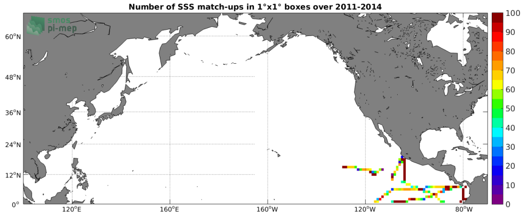
Figure 4: Number of SSS match-ups between TSG (GOSUD-Research-vessel) SSS and the Aquarius SSS L3 OR v5 - Monthly (NASA-GSFC) SSS product for the North Pacific Ocean Pi-MEP region over 1^\circ \times 1^\circ boxes and for the full satellite product period.
