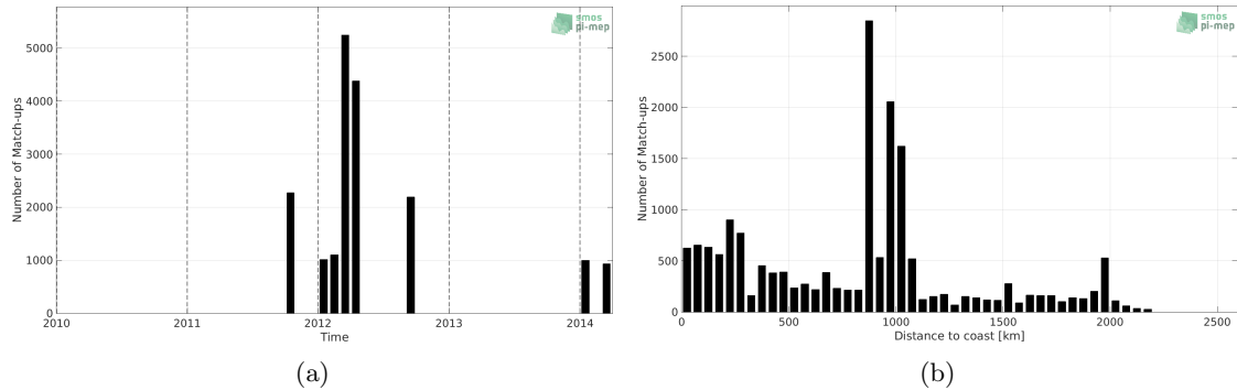
Figure 1: Number of match-ups between TSG (GOSUD-Research-vessel) and Aquarius SSS L3 OR v5 - Monthly (NASA-GSFC) SSS as a function of time (a) and as function of the distance to coast (b) over the North Pacific Ocean Pi-MEP region and for the full satellite product period.
