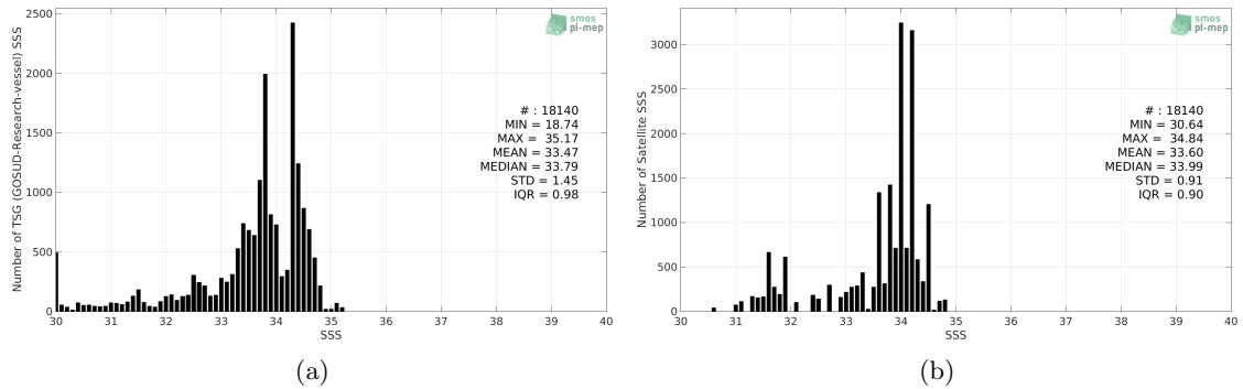
Figure 2: Histograms of SSS from TSG (GOSUD-Research-vessel) (a) and Aquarius SSS L3 OR v5 - Monthly (NASA-GSFC) (b) considering all match-up pairs per bins of 0.1 over the North Pacific Ocean Pi-MEP region and for the full satellite product period.
