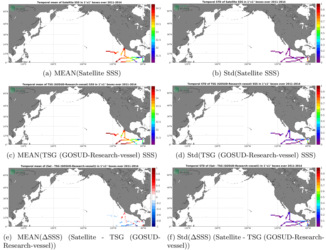
Figure 6: Temporal mean (left) and Std (right) of SSS from Aquarius SSS L3 OR v5 - Monthly (NASA-GSFC) (top), TSG (GOSUD-Research-vessel) ( in situ ) (middle), and of \Delta\text{SSS} (Satellite - TSG (GOSUD-Research-vessel)). Only match-up pairs are used to generate these maps.
