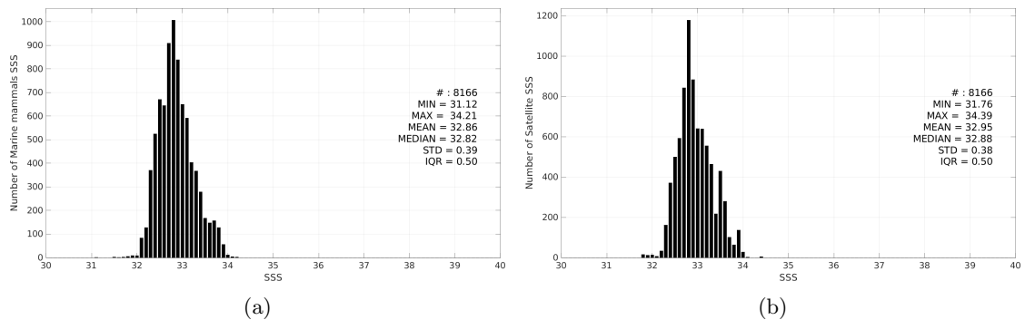
Figure 3: Histograms of SSS from Marine mammals (a) and Aquarius SSS L3 OR v5 - Monthly (NASA-GSFC) (b) considering all match-up pairs per bins of 0.1 over the North Pacific Ocean Pi-MEP region and for the full satellite product period.
