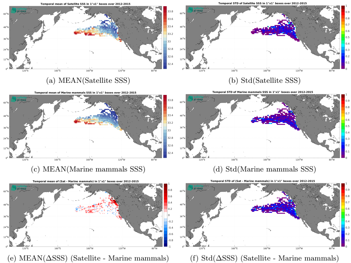
Figure 7: Temporal mean (left) and Std (right) of SSS from Aquarius SSS L3 OR v5 - Monthly (NASA-GSFC) (top), Marine mammals (middle), and of \Delta SSS (Satellite - Marine mammals). Only match-up pairs are used to generate these maps.
