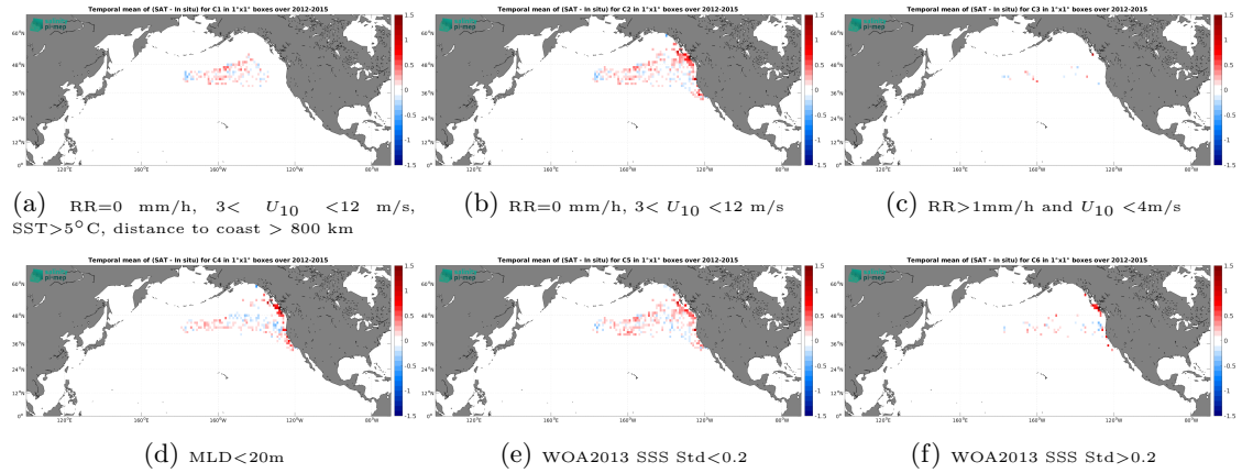
Figure 14: Temporal mean gridded over spatial boxes of size 1^\circ \times 1^\circ of \Delta SSS (Aquarius SSS L3 OR v5 - Monthly (NASA-GSFC) - Marine mammals) for 6 different subdatasets corresponding to:RR=0 mm/h, 3 < U_{10} < 12 m/s, SST>5°C, distance to coast > 800 km (a), RR=0 mm/h, 3 < U_{10} < 12 m/s (b), RR>1mm/h and U_{10} < 4 m/s (c),MLD<20m (d),WOA2013 SSS Std<0.2 (e),WOA2013 SSS Std>0.2 (f).
