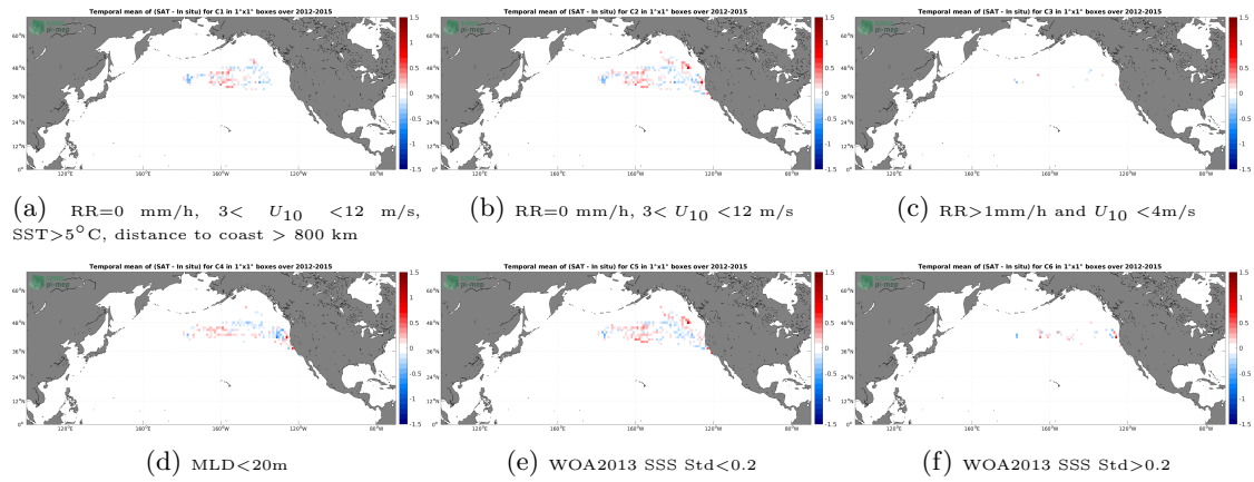
Figure 12: Temporal mean gridded over spatial boxes of size 1^\circ \times 1^\circ of \Delta SSS (Aquarius SSS L3 OR v5 - Monthly (NASA-GSFC) - Marine mammals) for 6 different subdatasets corresponding to:RR=0 mm/h, 3 < U_{10} < 12 m/s, SST >5^\circ C, distance to coast > 800 km (a), RR=0 mm/h, 3 < U_{10} < 12 m/s (b), RR >1 mm/h and U_{10} < 4 m/s (c),MLD <20 m (d),WOA2013 SSS Std <0.2 (e),WOA2013 SSS Std >0.2 (f).
