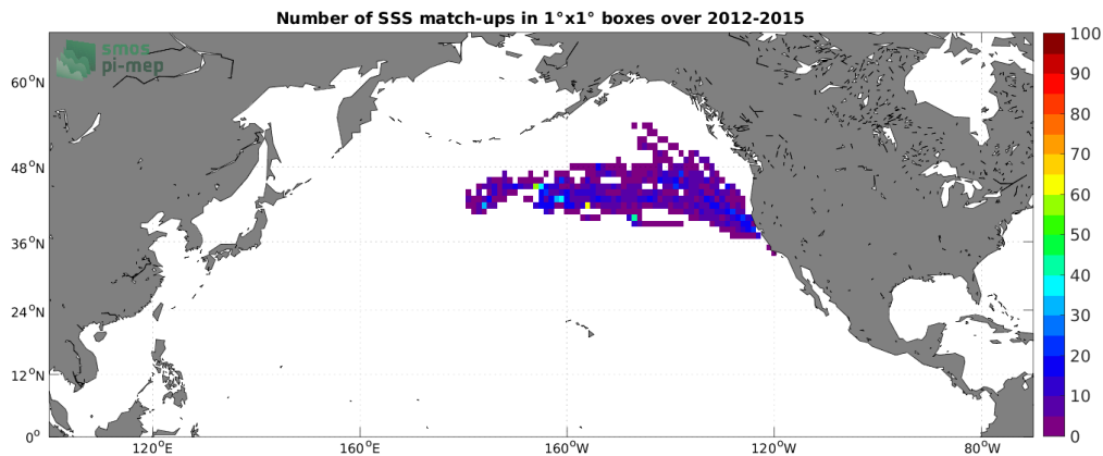
Figure 4: Number of SSS match-ups between Marine mammals SSS and the Aquarius SSS L3 OR v5 - Monthly (NASA-GSFC) SSS product for the North Pacific Ocean Pi-MEP region over 1^\circ \times 1^\circ boxes and for the full satellite product period.
