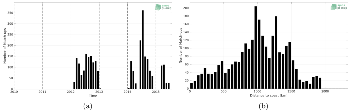
Figure 1: Number of match-ups between Marine mammals and Aquarius SSS L3 OR v5 - Monthly (NASA-GSFC) SSS as a function of time (a) and as function of the distance to coast (b) over the North Pacific Ocean Pi-MEP region and for the full satellite product period.
