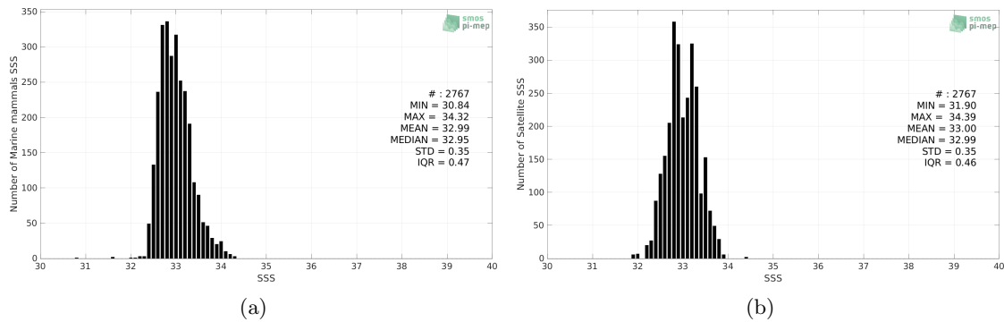
Figure 2: Histograms of SSS from Marine mammals (a) and Aquarius SSS L3 OR v5 - Monthly (NASA-GSFC) (b) considering all match-up pairs per bins of 0.1 over the North Pacific Ocean Pi-MEP region and for the full satellite product period.
