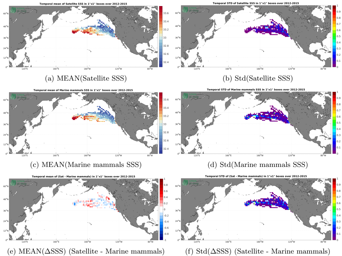
Figure 6: Temporal mean (left) and Std (right) of SSS from Aquarius SSS L3 OR v5 - Monthly (NASA-GSFC) (top), Marine mammals (middle), and of \Delta SSS (Satellite - Marine mammals). Only match-up pairs are used to generate these maps.
