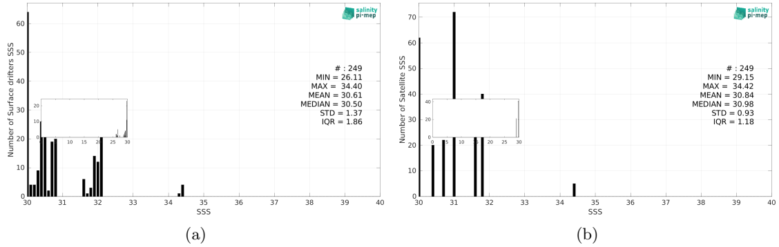
Figure 3: Histograms of SSS from Surface drifters (a) and Aquarius SSS L3 OR v5 - Monthly (NASA-GSFC) (b) considering all match-up pairs per bins of 0.1 over the North Pacific Ocean Pi-MEP region and for the full satellite product period.
