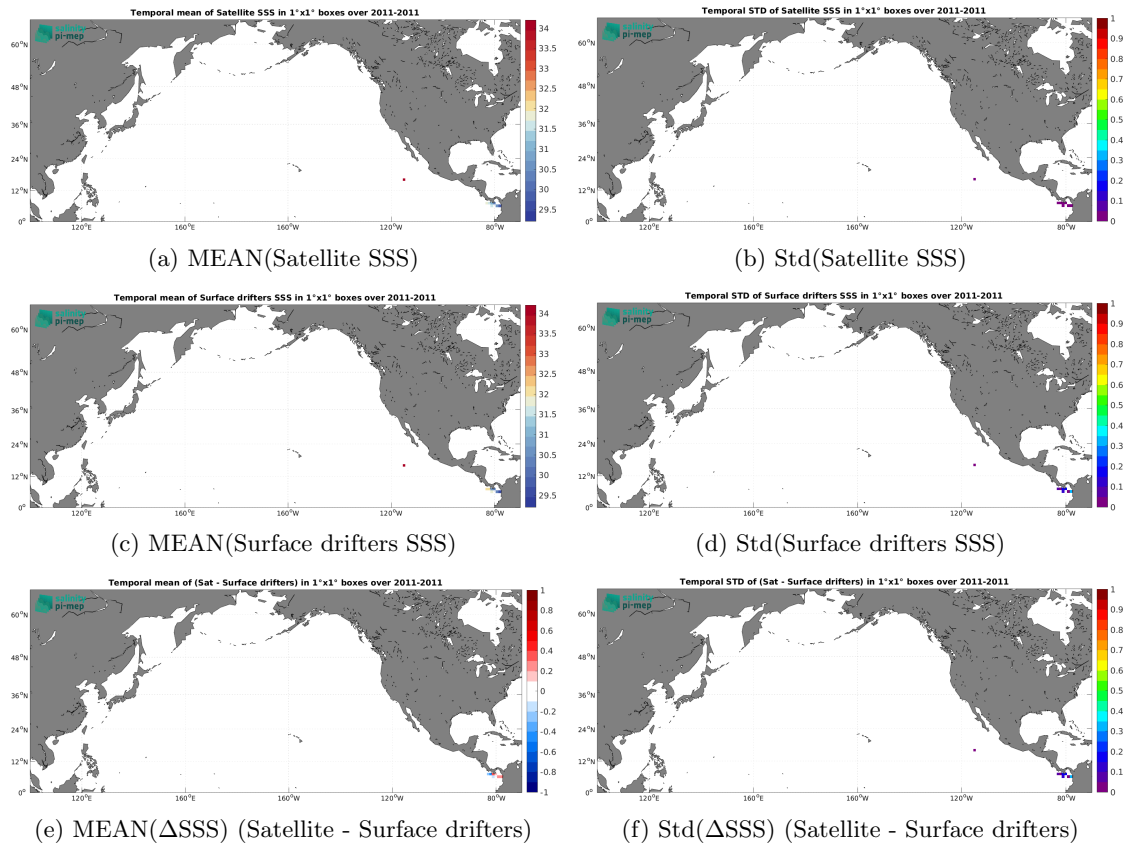
Figure 6: Temporal mean (left) and Std (right) of SSS from Aquarius SSS L3 OR v5 - Monthly (NASA-GSFC) (top), Surface drifters (middle), and of \Delta SSS (Satellite - Surface drifters). Only match-up pairs are used to generate these maps.
