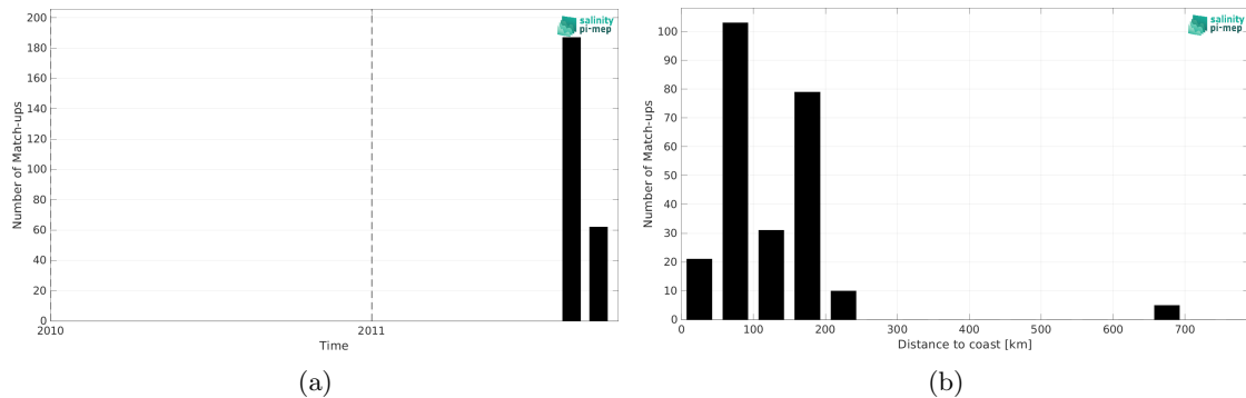
Figure 2: Number of match-ups between Surface drifters and Aquarius SSS L3 OR v5 - Monthly (NASA-GSFC) SSS as a function of time (a) and as function of the distance to coast (b) over the North Pacific Ocean Pi-MEP region and for the full satellite product period.
