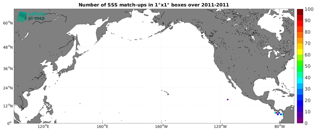
Figure 4: Number of SSS match-ups between Surface drifters SSS and the Aquarius SSS L3 OR v5 - Monthly (NASA-GSFC) SSS product for the North Pacific Ocean Pi-MEP region over 1^\circ \times 1^\circ boxes and for the full satellite product period.
